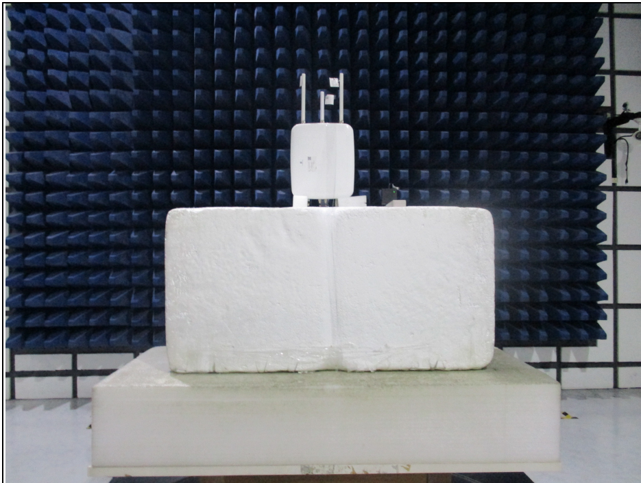
EIRP Power Test / Radiated Emission Test above 1GHz
