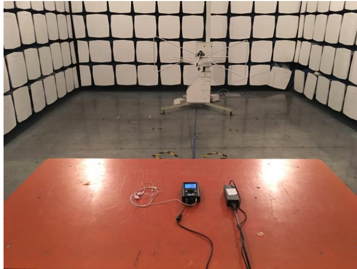
Radiated
