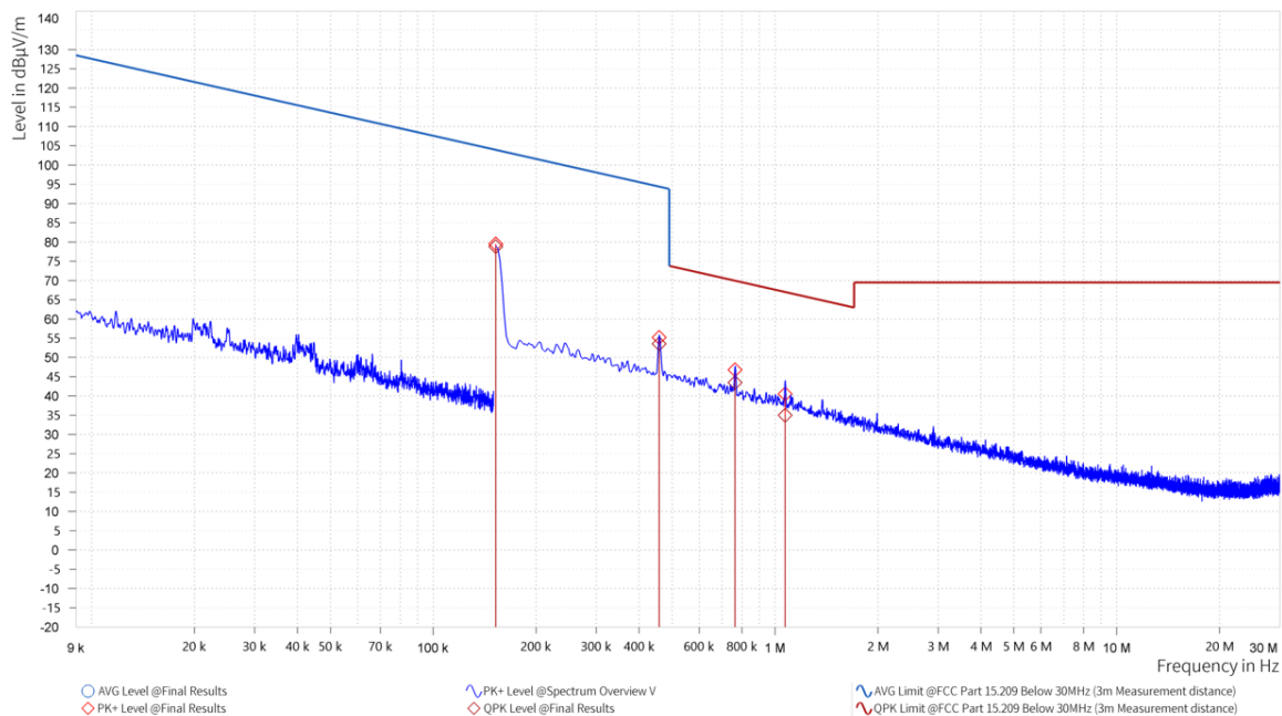
Plot 5. Spurious Emissions 9kHz – 30MHz, 90 degrees Loop Antenna
