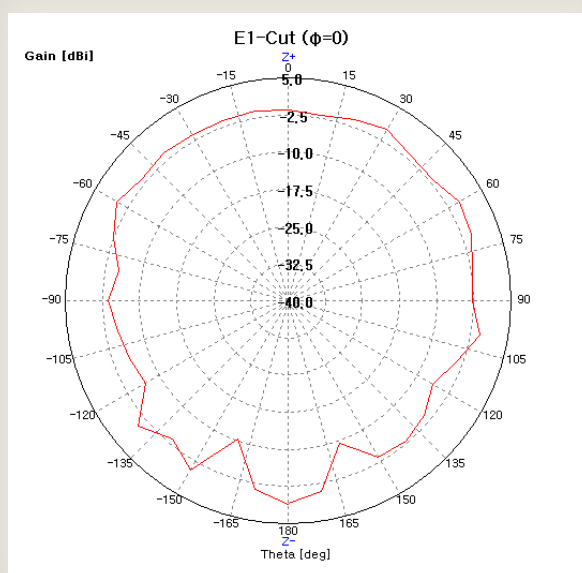
[Elevation1 plane @2442MHz]
