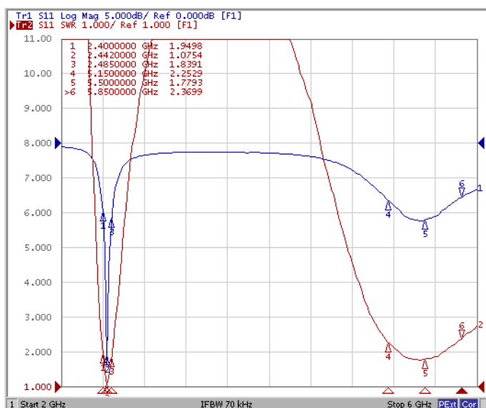
Measured VSWR and Return-loss
