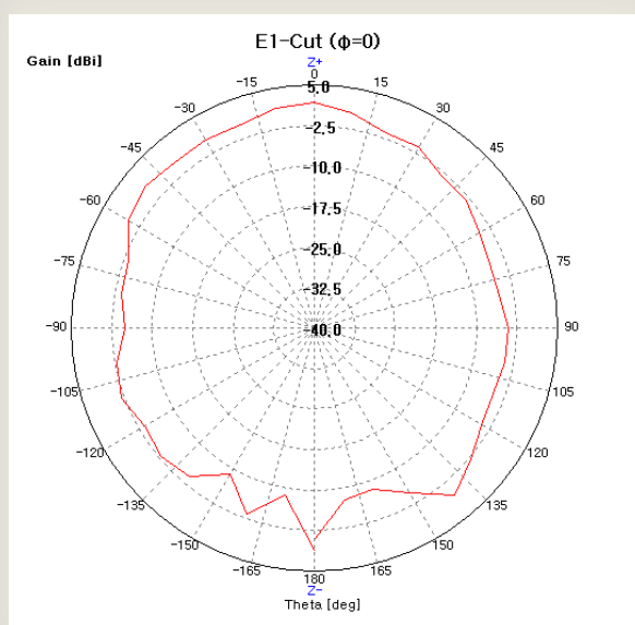
[Elevation1 plane @5500MHz ]
