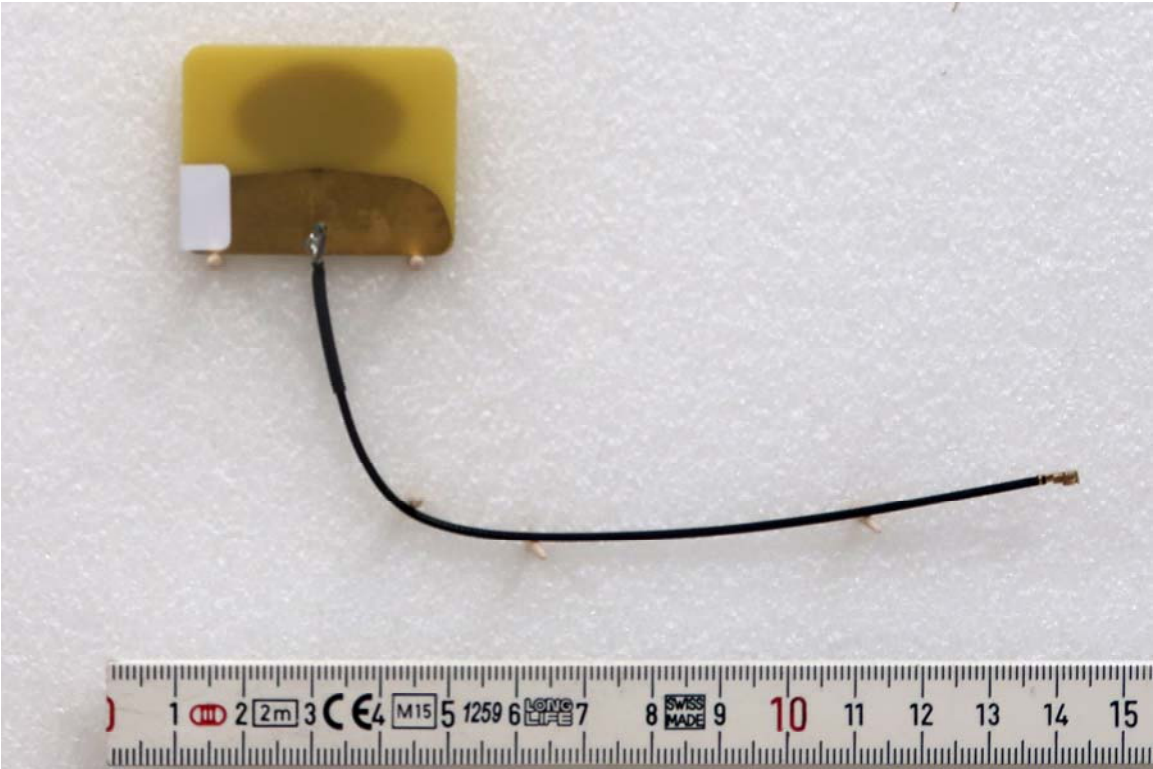
Medium Antenna Rear
