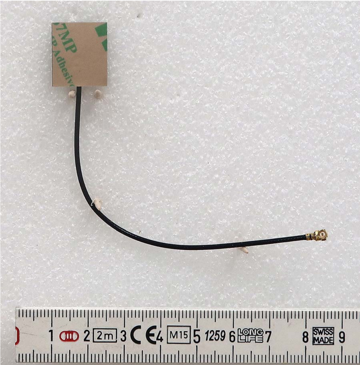
Small Antenna Rear
