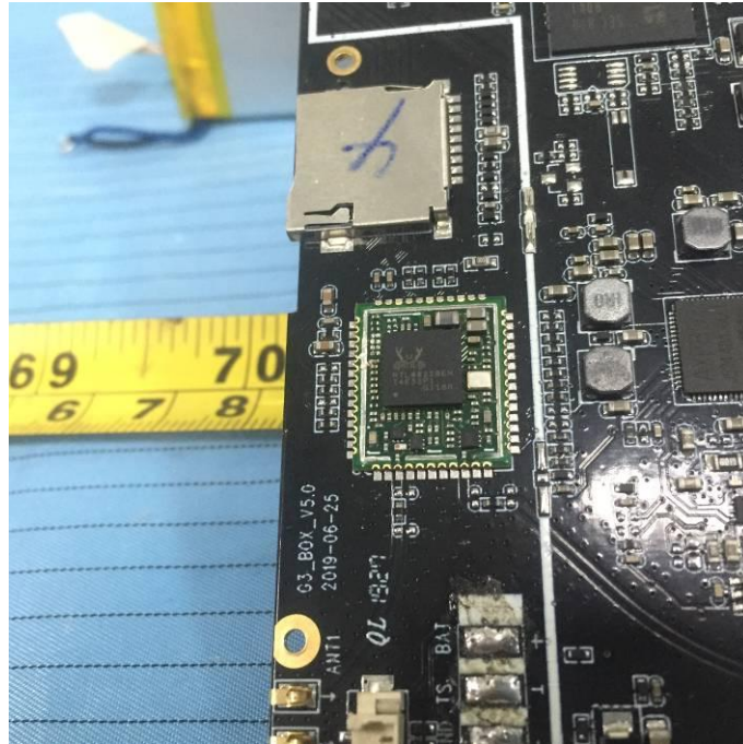
EUT – Main Chip 2 View
