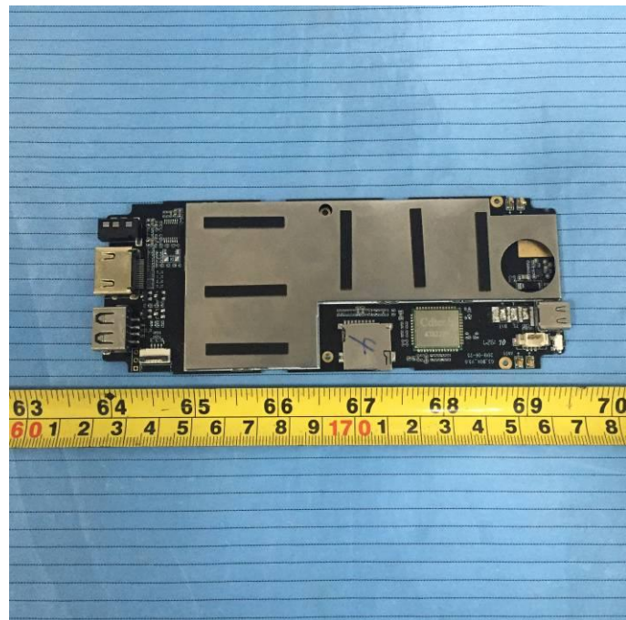
EUT – Main Board Top Shielding off View
