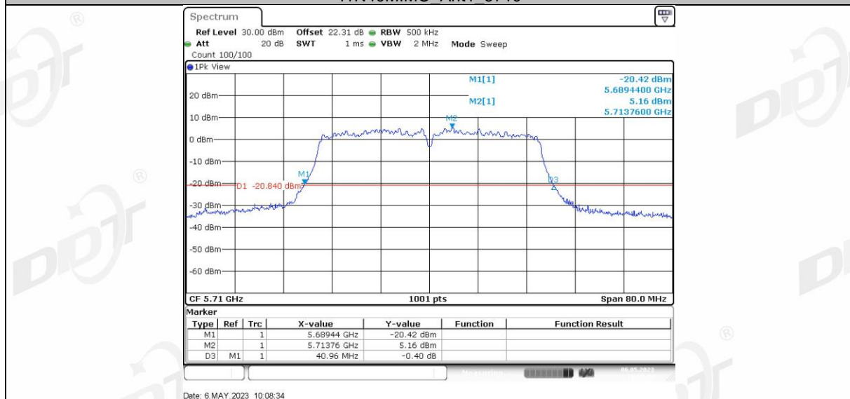
11N40MIMO Ant2 5710
