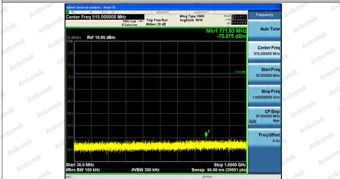
3DH5_Ant1_2402_30~1000
