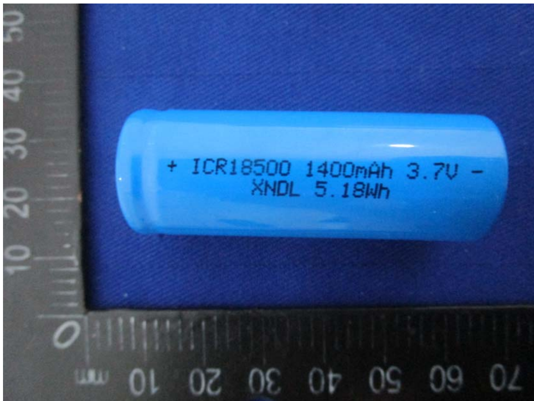
Battery
