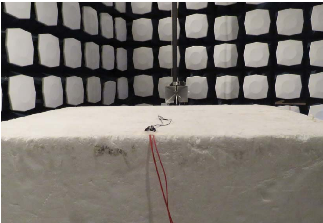
Picture 2 Radiated Emission Test Setup
