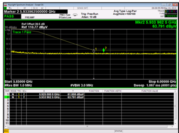
Band IV 11ac80 CH155 Peak
