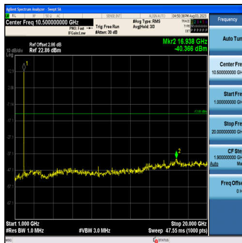
Band2-15MHz-16QAM-19125-75RB#0-Range2:1000~20000MHz
