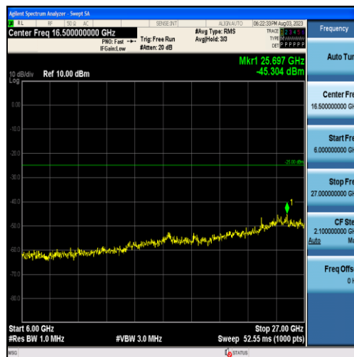
Band7-5MHz-16QAM-21100-25RB#0-Range3:6000~27000MHz
