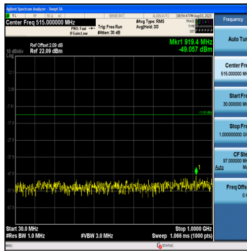
Band25-3MHz-QPSK-26675-15RB#0-Range1:30~1000MHz
