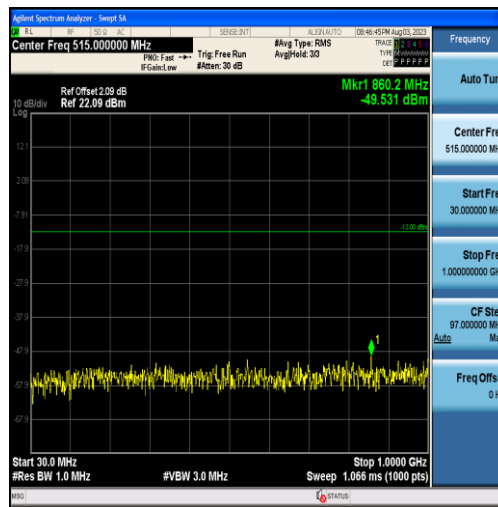
Band25-1.4MHz-16QAM-26047-6RB#0-Range1:30~1000MHz
