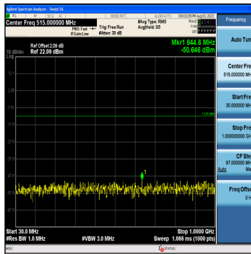
Band25-5MHz-QPSK-26665-25RB#0-Range1:30~1000MHz
