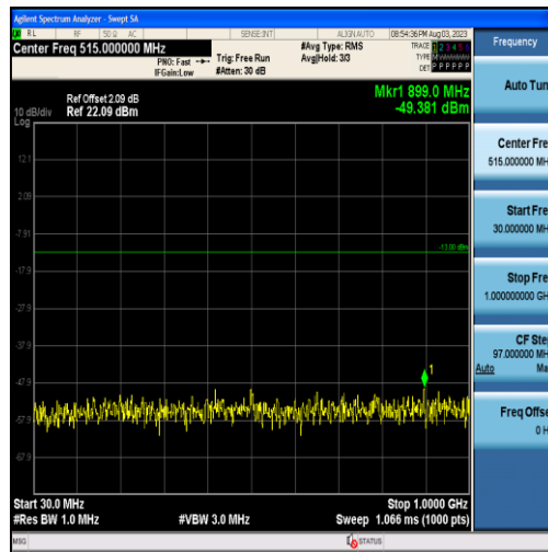
Band25-3MHz-16QAM-26365-15RB#0-Range1:30~1000MHz
