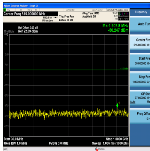
Band25-3MHz-QPSK-26365-15RB#0-Range1:30~1000MHz
