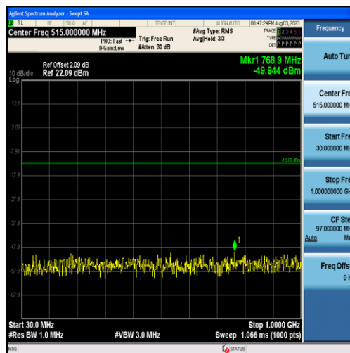
Band25-1.4MHz-16QAM-26683-6RB#0-Range1:30~1000MHz
