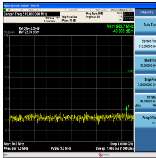
Band25-5MHz-16QAM-26065-25RB#0-Range1:30~1000MHz
