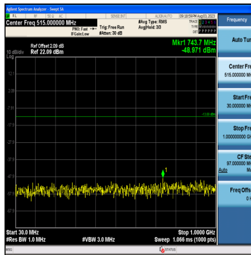
Band25-15MHz-QPSK-26615-75RB#0-Range1:30~1000MHz
