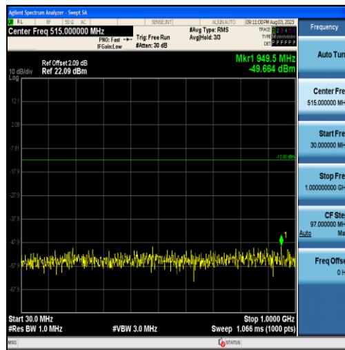
Band25-10MHz-QPSK-26640-50RB#0-Range1:30~1000MHz
