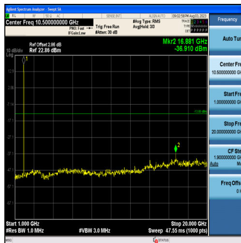
Band25-5MHz-16QAM-26365-25RB#0-Range2:1000~20000MHz
