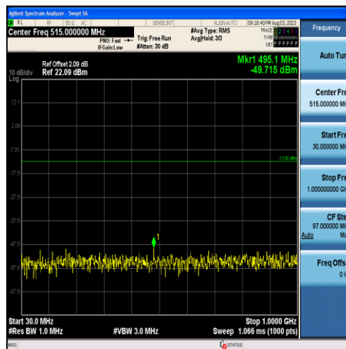
Band25-15MHz-QPSK-26365-75RB#0-Range1:30~1000MHz
