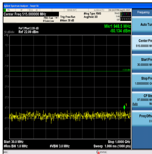
Band25-15MHz-16QAM-26615-75RB#0-Range1:30~1000MHz
