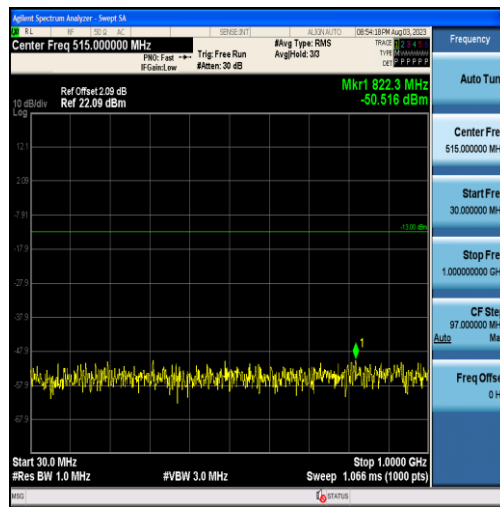
Band25-3MHz-16QAM-26055-15RB#0-Range1:30~1000MHz
