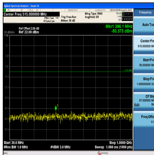
Band25-3MHz-16QAM-26675-15RB#0-Range1:30~1000MHz
