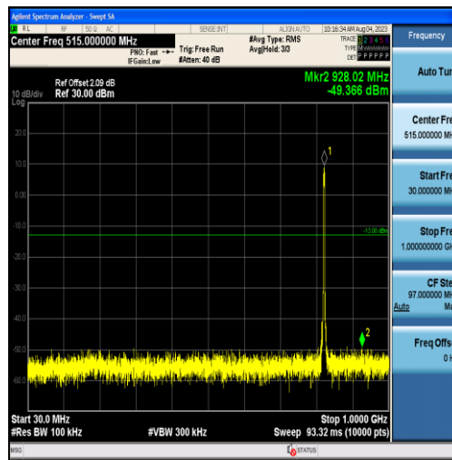
Band26-3MHz-16QAM-26805-15RB#0-Range1:30~1000MHz
