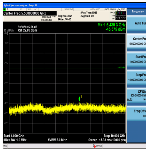
Band26-5MHz-16QAM-26765-25RB#0-Range2:1000~10000MHz
