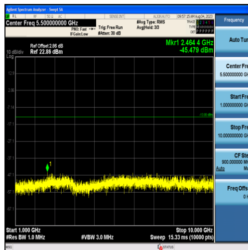
Band26-5MHz-16QAM-26740-25RB#0-Range2:1000~10000MHz
