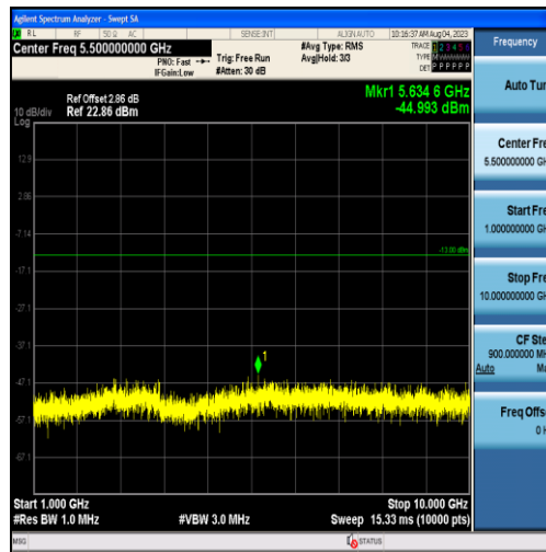
Band26-3MHz-16QAM-26805-15RB#0-Range2:1000~10000MHz
