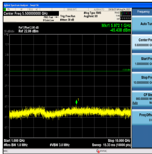
Band26-5MHz-16QAM-26715-25RB#0-Range2:1000~10000MHz
