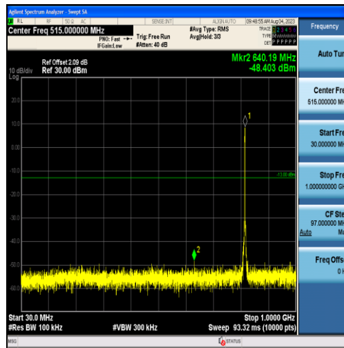
Band26-3MHz-16QAM-26740-15RB#0-Range1:30~1000MHz
