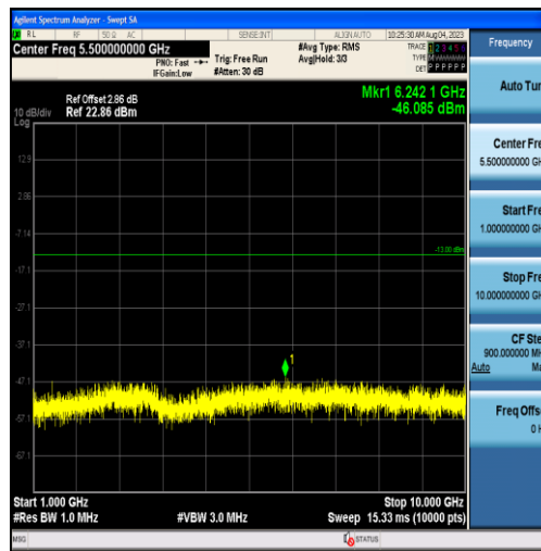
Band26-5MHz-16QAM-27015-25RB#0-Range2:1000~10000MHz
