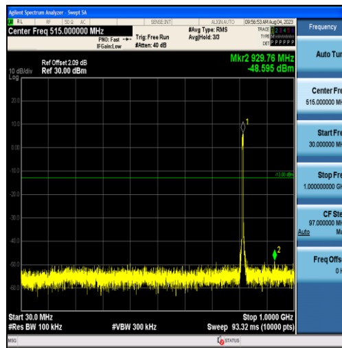
Band26-5MHz-16QAM-26715-25RB#0-Range1:30~1000MHz
