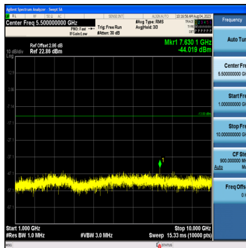
Band26-3MHz-16QAM-26915-15RB#0-Range2:1000~10000MHz
