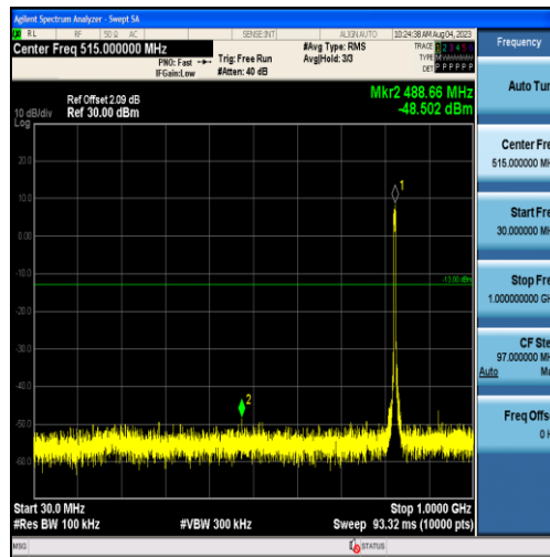
Band26-5MHz-QPSK-26815-25RB#0-Range1:30~1000MHz
