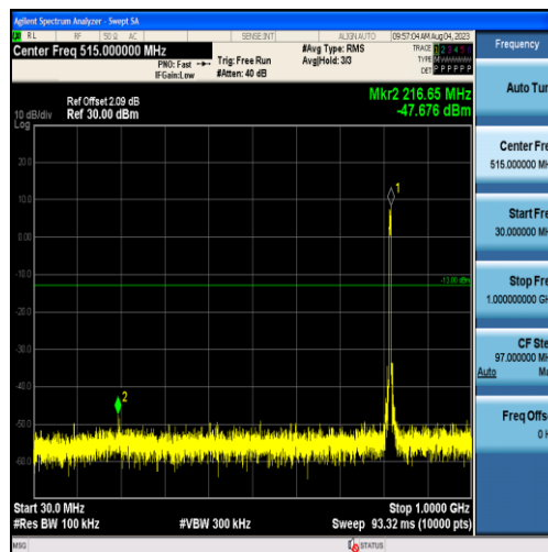
Band26-5MHz-QPSK-26740-25RB#0-Range1:30~1000MHz
