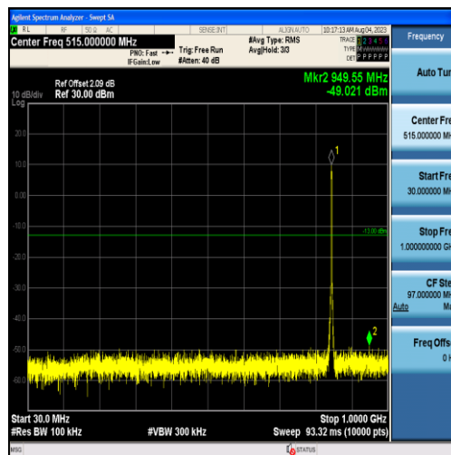
Band26-3MHz-16QAM-27025-15RB#0-Range1:30~1000MHz
