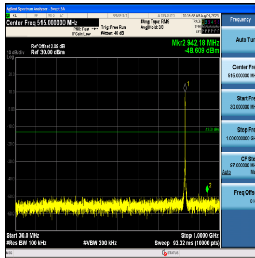
Band26-3MHz-16QAM-26915-15RB#0-Range1:30~1000MHz
