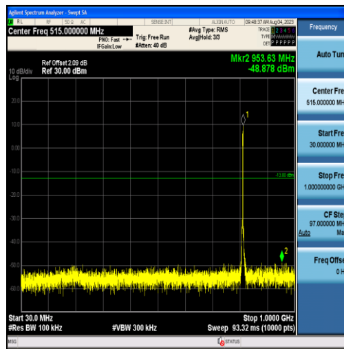
Band26-3MHz-16QAM-26705-15RB#0-Range1:30~1000MHz
