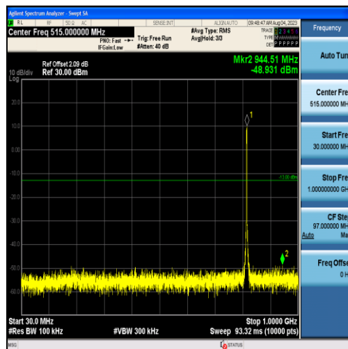
Band26-3MHz-QPSK-26740-15RB#0-Range1:30~1000MHz
