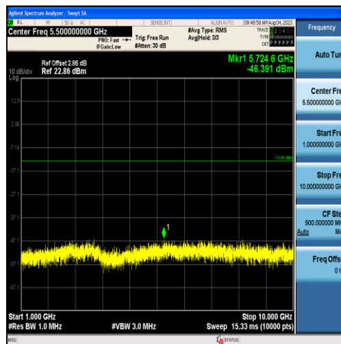
Band26-3MHz-16QAM-26740-15RB#0-Range2:1000~10000MHz
