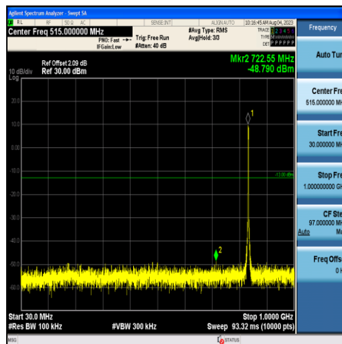
Band26-3MHz-QPSK-26915-15RB#0-Range1:30~1000MHz
