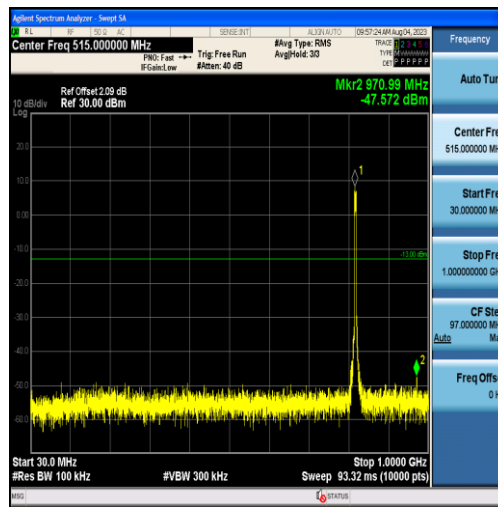
Band26-5MHz-QPSK-26765-25RB#0-Range1:30~1000MHz
