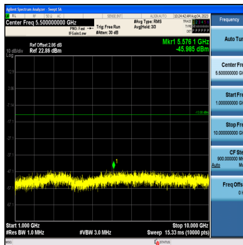
Band26-5MHz-QPSK-26815-25RB#0-Range2:1000~10000MHz
