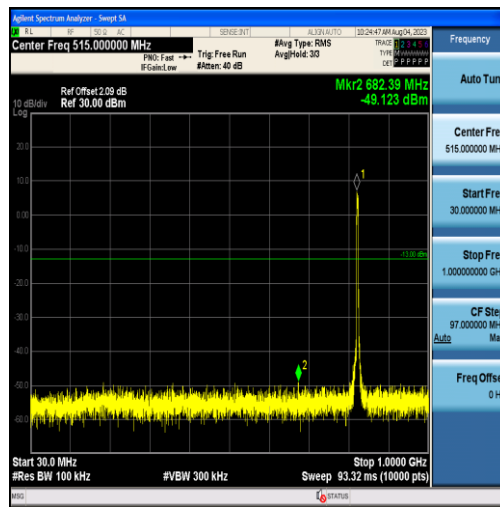
Band26-5MHz-16QAM-26815-25RB#0-Range1:30~1000MHz
