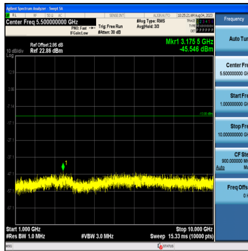
Band26-5MHz-QPSK-27015-25RB#0-Range2:1000~10000MHz
