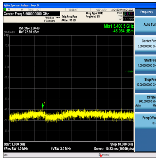
Band26-5MHz-16QAM-26815-25RB#0-Range2:1000~10000MHz
