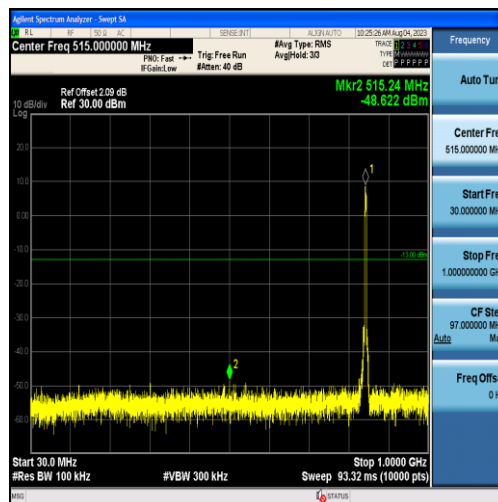
Band26-5MHz-16QAM-27015-25RB#0-Range1:30~1000MHz
