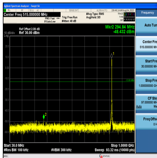
Band26-3MHz-16QAM-26775-15RB#0-Range1:30~1000MHz
