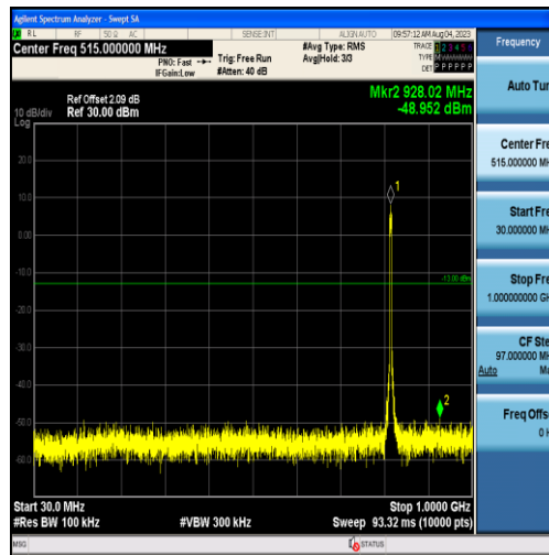
Band26-5MHz-16QAM-26740-25RB#0-Range1:30~1000MHz
