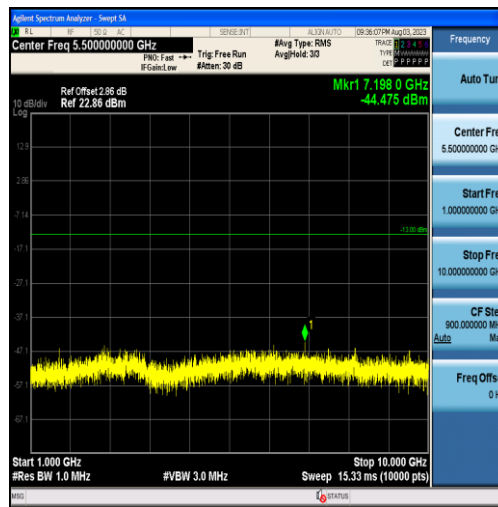
Band26-1.4MHz-16QAM-26783-6RB#0-Range2:1000~10000MHz
