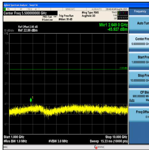
Band26-3MHz-16QAM-26705-15RB#0-Range2:1000~10000MHz
