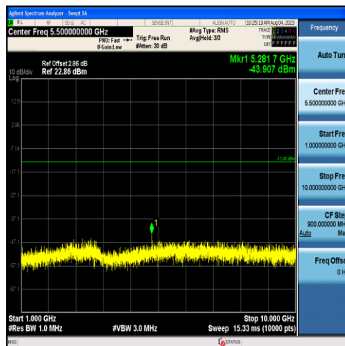
Band26-5MHz-16QAM-26915-25RB#0-Range2:1000~10000MHz
