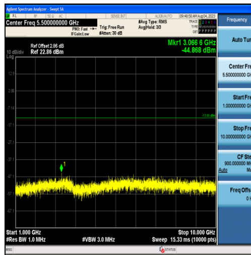
Band26-3MHz-QPSK-26740-15RB#0-Range2:1000~10000MHz
