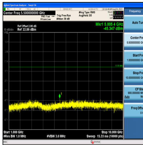
Band26-3MHz-QPSK-26915-15RB#0-Range2:1000~10000MHz
