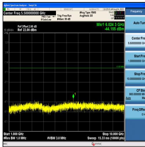
Band26-5MHz-QPSK-26915-25RB#0-Range2:1000~10000MHz
