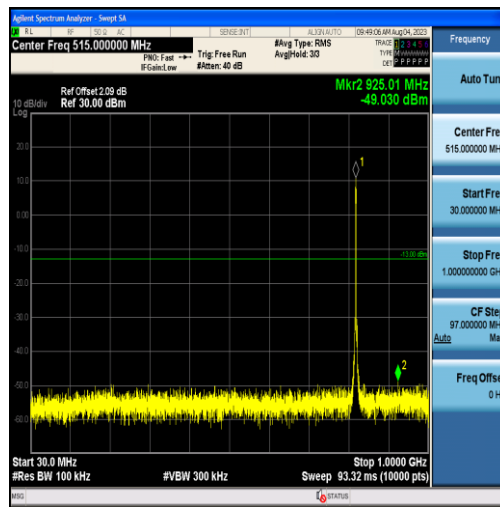
Band26-3MHz-QPSK-26775-15RB#0-Range1:30~1000MHz
