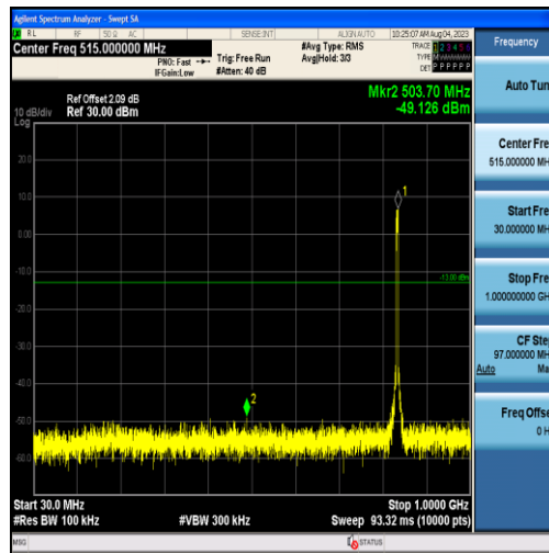
Band26-5MHz-16QAM-26915-25RB#0-Range1:30~1000MHz
