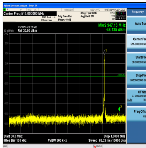
Band26-5MHz-16QAM-26765-25RB#0-Range1:30~1000MHz
