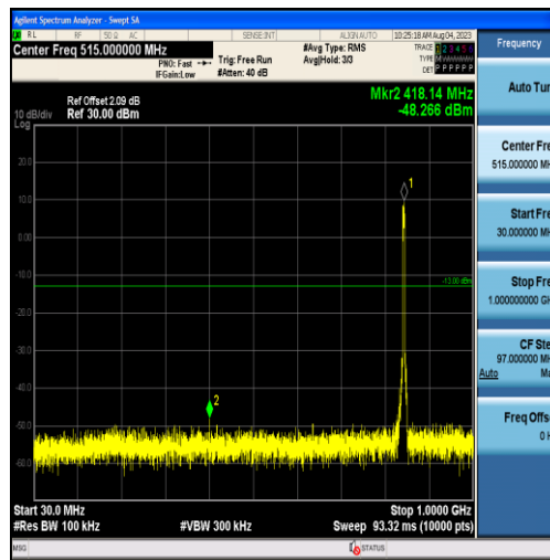
Band26-5MHz-QPSK-27015-25RB#0-Range1:30~1000MHz
