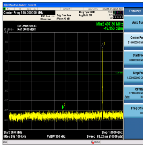
Band26-1.4MHz-QPSK-26797-6RB#0-Range1:30~1000MHz
