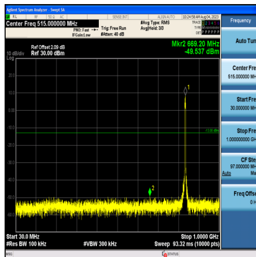
Band26-5MHz-QPSK-26915-25RB#0-Range1:30~1000MHz
