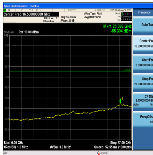
Band38-10MHz-16QAM-37800-50RB#0-Range3:6000~27000MHz
