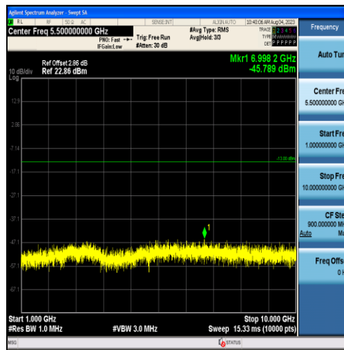
Band26-15MHz-16QAM-26865-75RB#0-Range2:1000~10000MHz
