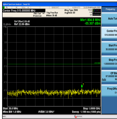
Band38-10MHz-QPSK-37800-50RB#0-Range1:30~1000MHz
