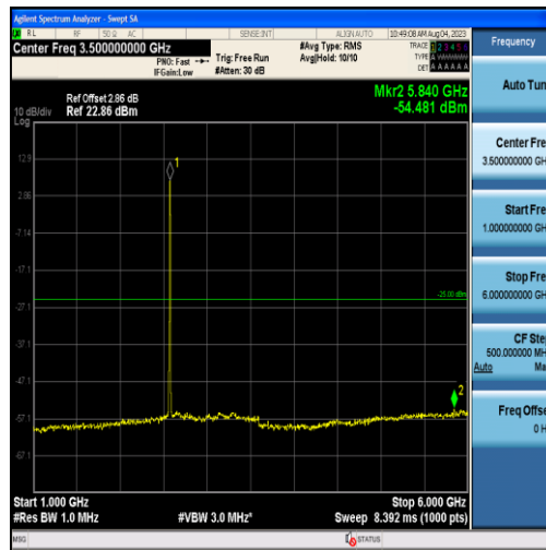
Band38-5MHz-QPSK-37775-25RB#0-Range2:1000~6000MHz
