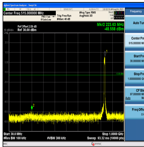
Band26-10MHz-QPSK-26915-50RB#0-Range1:30~1000MHz
