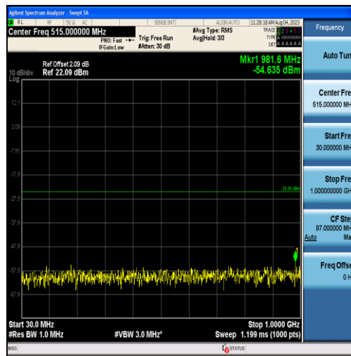
Band38-10MHz-QPSK-38200-50RB#0-Range1:30~1000MHz
