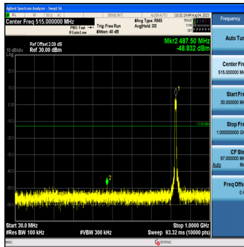
Band26-10MHz-16QAM-26840-50RB#0-Range1:30~1000MHz
