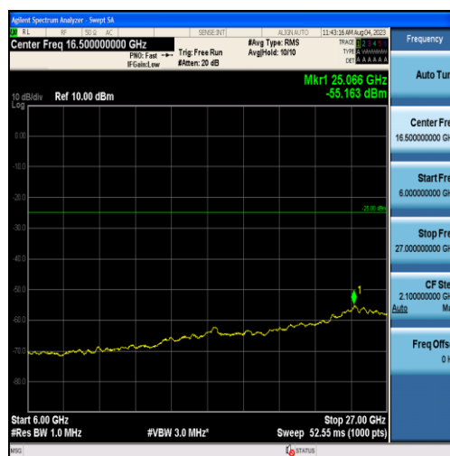
Band38-15MHz-16QAM-38175-75RB#0-Range3:6000~27000MHz
