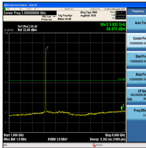
Band38-10MHz-16QAM-37800-50RB#0-Range2:1000~6000MHz
