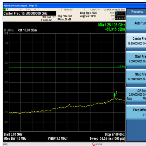
Band38-15MHz-16QAM-37825-75RB#0-Range3:6000~27000MHz
