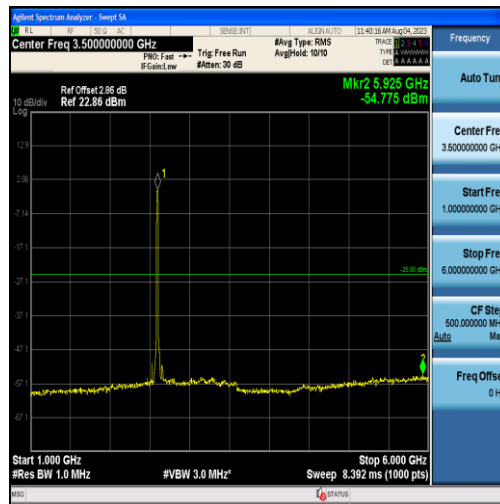
Band38-15MHz-16QAM-38000-75RB#0-Range2:1000~6000MHz
