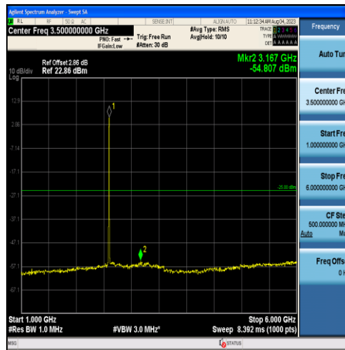
Band38-5MHz-16QAM-38000-25RB#0-Range2:1000~6000MHz
