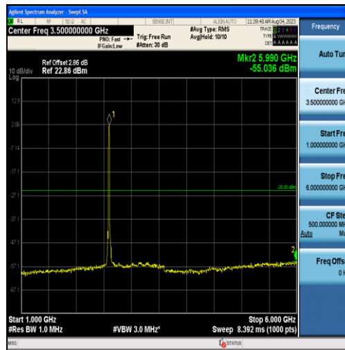
Band38-15MHz-QPSK-38000-75RB#0-Range2:1000~6000MHz
