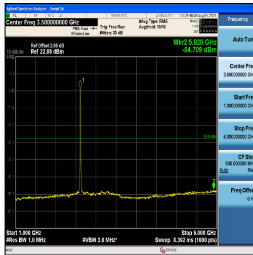
Band38-10MHz-16QAM-38200-50RB#0-Range2:1000~6000MHz
