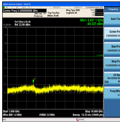
Band26-15MHz-QPSK-26865-75RB#0-Range2:1000~10000MHz
