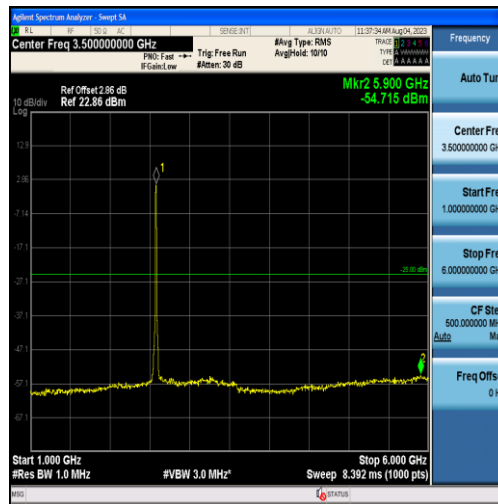
Band38-15MHz-QPSK-37825-75RB#0-Range2:1000~6000MHz
