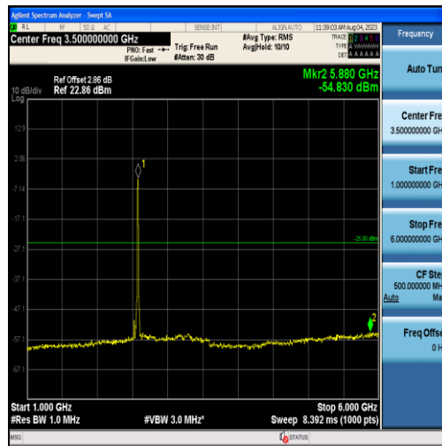
Band38-15MHz-16QAM-37825-75RB#0-Range2:1000~6000MHz
