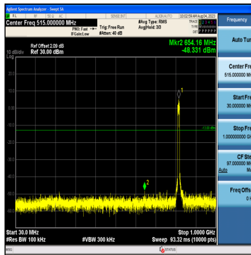
Band26-10MHz-16QAM-26740-50RB#0-Range1:30~1000MHz
