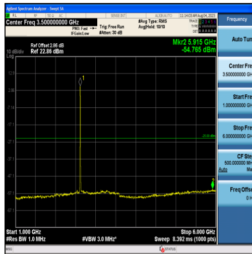
Band38-5MHz-16QAM-38225-25RB#0-Range2:1000~6000MHz
