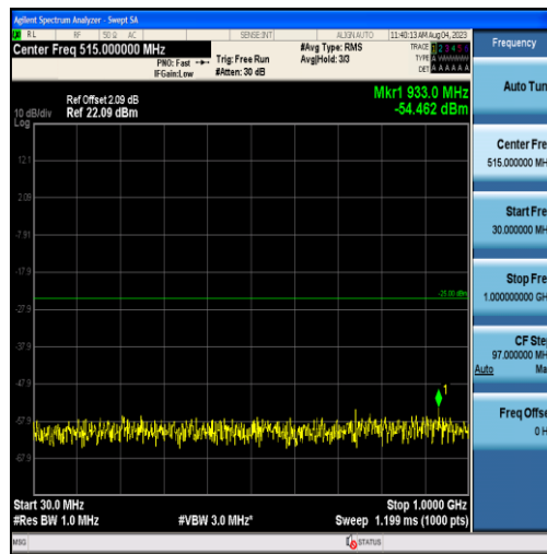
Band38-15MHz-16QAM-38000-75RB#0-Range1:30~1000MHz
