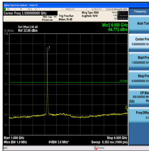
Band38-15MHz-QPSK-38175-75RB#0-Range2:1000~6000MHz
