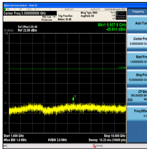
Band26-15MHz-QPSK-26965-75RB#0-Range2:1000~10000MHz
