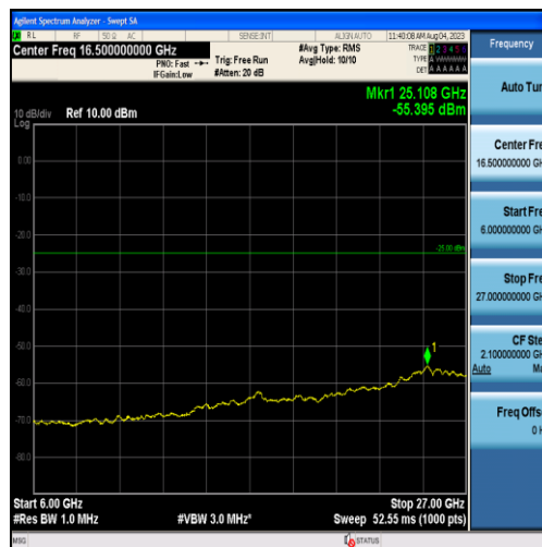
Band38-15MHz-QPSK-38000-75RB#0-Range3:6000~27000MHz
