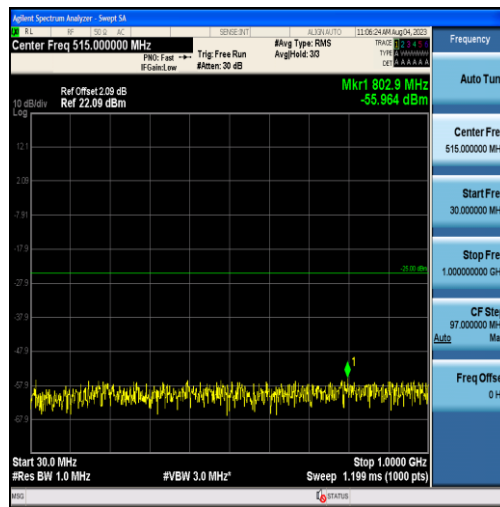
Band38-5MHz-QPSK-38000-25RB#0-Range1:30~1000MHz
