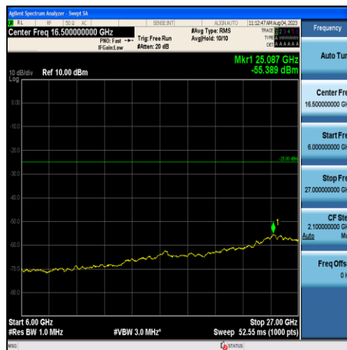
Band38-5MHz-16QAM-38000-25RB#0-Range3:6000~27000MHz
