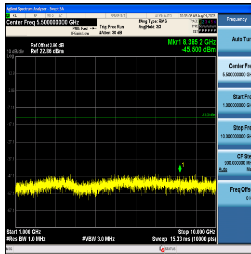
Band26-10MHz-16QAM-26990-50RB#0-Range2:1000~10000MHz
