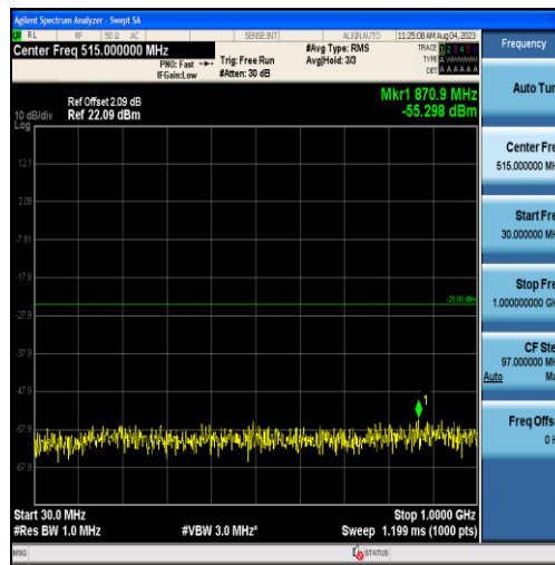
Band38-10MHz-16QAM-37800-50RB#0-Range1:30~1000MHz
