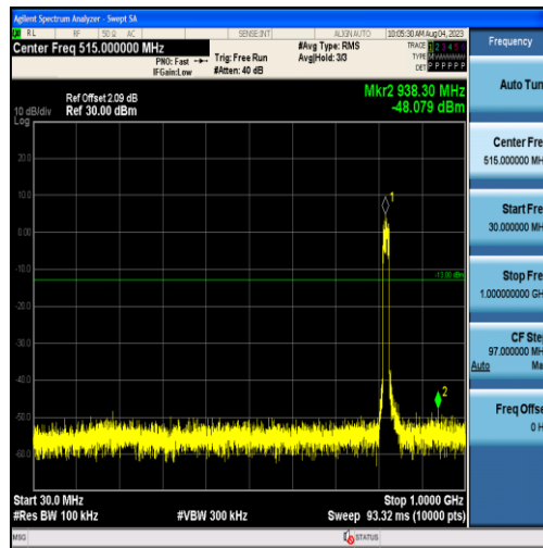
Band26-15MHz-16QAM-26765-75RB#0-Range1:30~1000MHz
