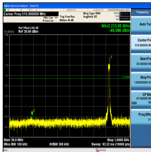
Band26-15MHz-16QAM-26865-75RB#0-Range1:30~1000MHz
