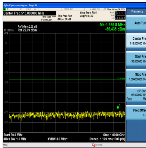
Band38-10MHz-16QAM-38200-50RB#0-Range1:30~1000MHz
