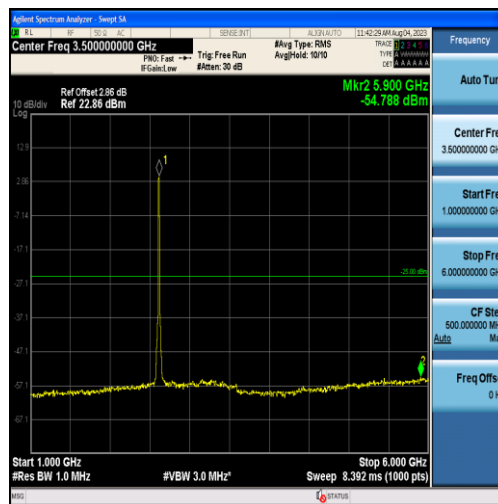
Band38-15MHz-16QAM-38175-75RB#0-Range2:1000~6000MHz
