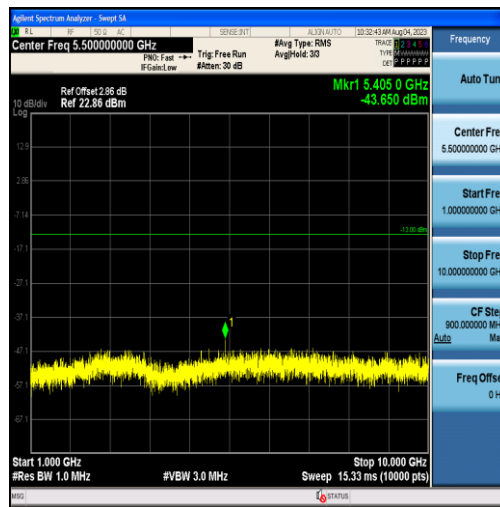
Band26-10MHz-16QAM-26915-50RB#0-Range2:1000~10000MHz
