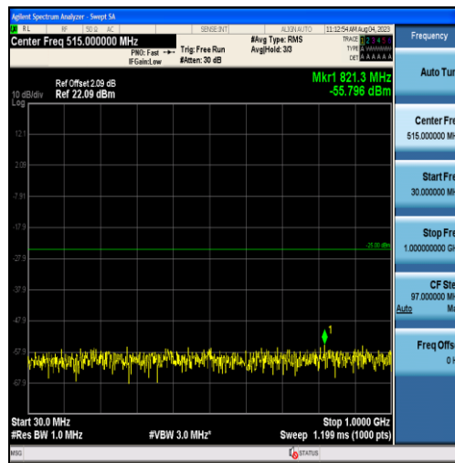
Band38-5MHz-QPSK-38225-25RB#0-Range1:30~1000MHz
