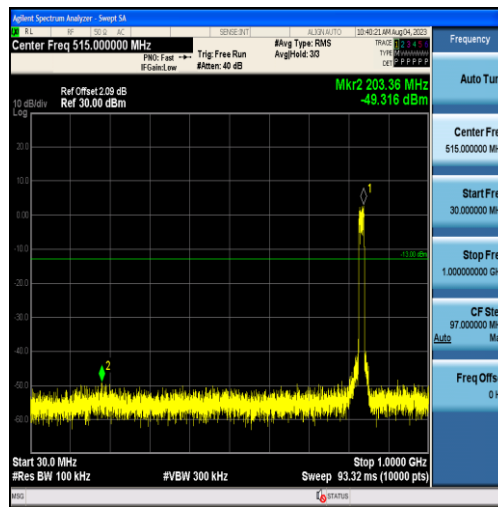
Band26-15MHz-16QAM-26915-75RB#0-Range1:30~1000MHz
