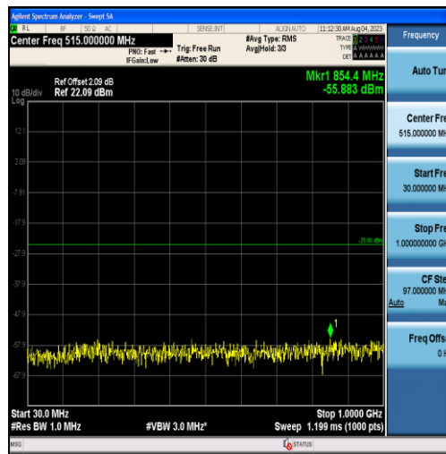
Band38-5MHz-16QAM-38000-25RB#0-Range1:30~1000MHz
