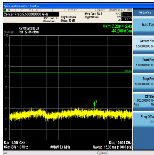
Band26-15MHz-16QAM-26765-75RB#0-Range2:1000~10000MHz
