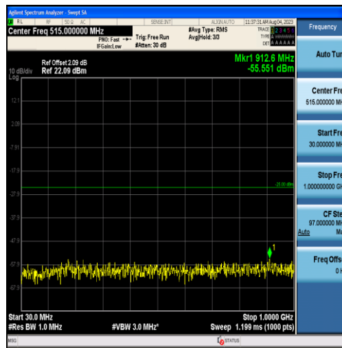
Band38-15MHz-QPSK-37825-75RB#0-Range1:30~1000MHz
