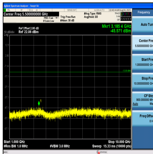
Band26-15MHz-16QAM-26965-75RB#0-Range2:1000~10000MHz
