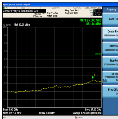
Band38-10MHz-16QAM-38000-50RB#0-Range3:6000~27000MHz
