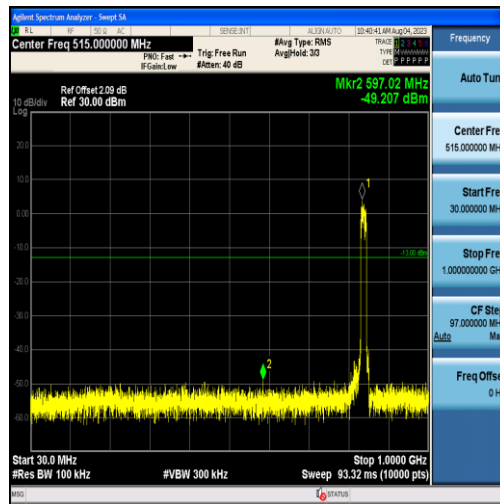
Band26-15MHz-16QAM-26965-75RB#0-Range1:30~1000MHz
