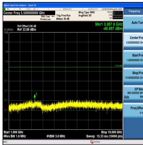
Band26-15MHz-QPSK-26765-75RB#0-Range2:1000~10000MHz
