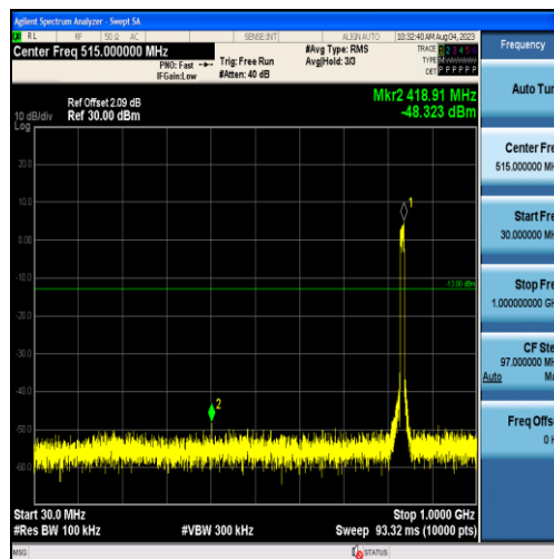
Band26-10MHz-16QAM-26915-50RB#0-Range1:30~1000MHz
