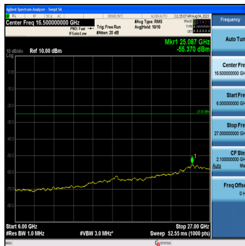
Band38-5MHz-16QAM-38225-25RB#0-Range3:6000~27000MHz
