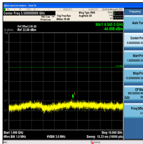
Band26-15MHz-QPSK-26915-75RB#0-Range2:1000~10000MHz
