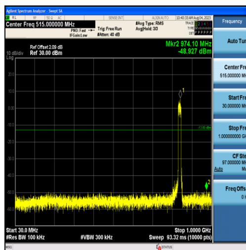
Band26-15MHz-QPSK-26965-75RB#0-Range1:30~1000MHz
