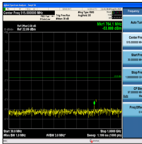
Band38-15MHz-QPSK-38175-75RB#0-Range1:30~1000MHz
