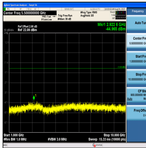
Band26-10MHz-16QAM-26740-50RB#0-Range2:1000~10000MHz
