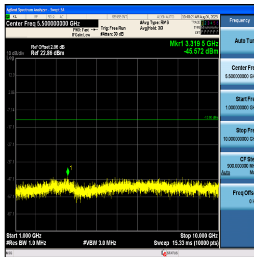
Band26-15MHz-16QAM-26915-75RB#0-Range2:1000~10000MHz
