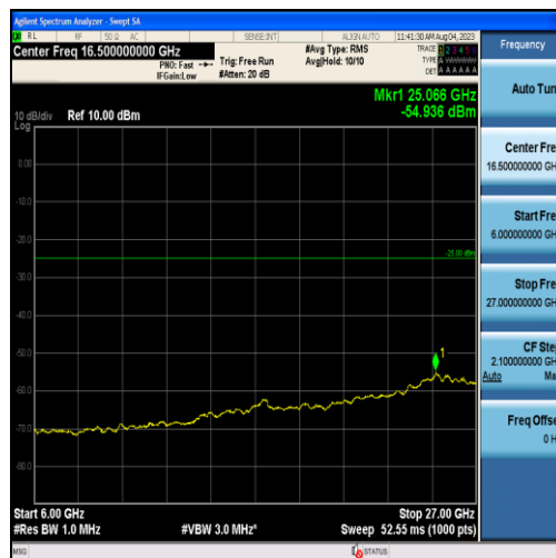
Band38-15MHz-16QAM-38000-75RB#0-Range3:6000~27000MHz
