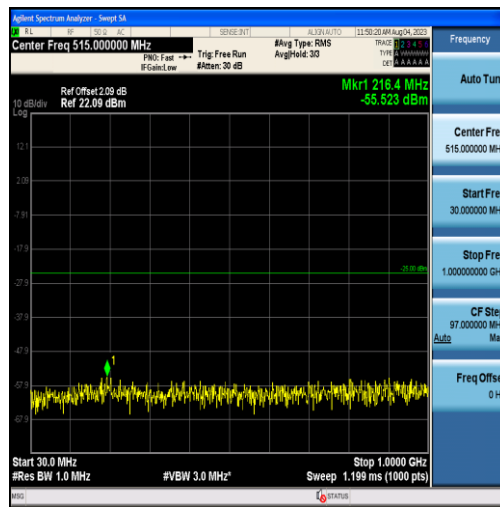
Band38-20MHz-QPSK-37850-100RB#0-Range1:30~1000MHz
