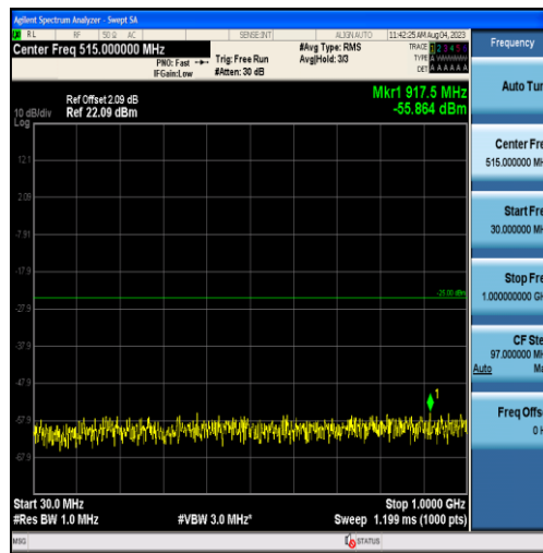
Band38-15MHz-16QAM-38175-75RB#0-Range1:30~1000MHz
