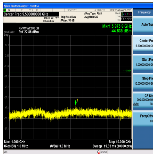
Band26-10MHz-16QAM-26840-50RB#0-Range2:1000~10000MHz
