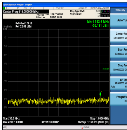
Band38-15MHz-QPSK-38000-75RB#0-Range1:30~1000MHz
