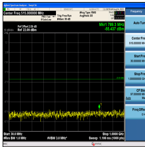
Band38-15MHz-16QAM-37825-75RB#0-Range1:30~1000MHz
