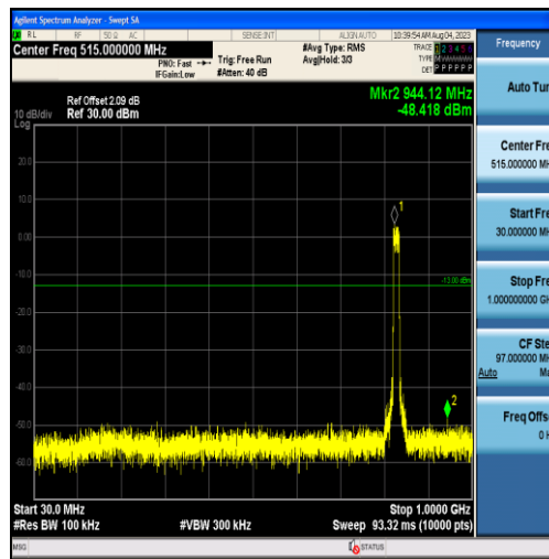
Band26-15MHz-QPSK-26865-75RB#0-Range1:30~1000MHz
