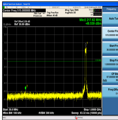
Band26-15MHz-QPSK-26915-75RB#0-Range1:30~1000MHz
