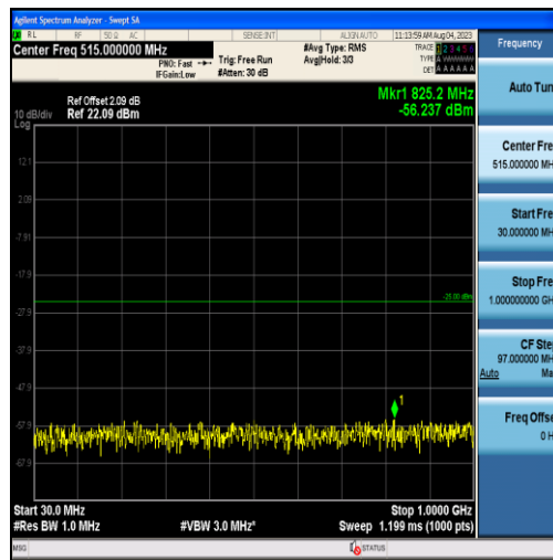
Band38-5MHz-16QAM-38225-25RB#0-Range1:30~1000MHz
