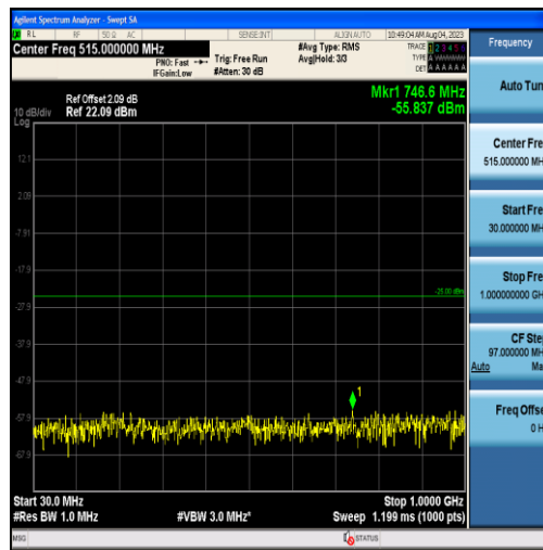
Band38-5MHz-QPSK-37775-25RB#0-Range1:30~1000MHz
