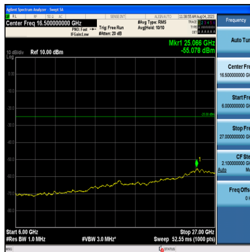
Band38-15MHz-QPSK-37825-75RB#0-Range3:6000~27000MHz
