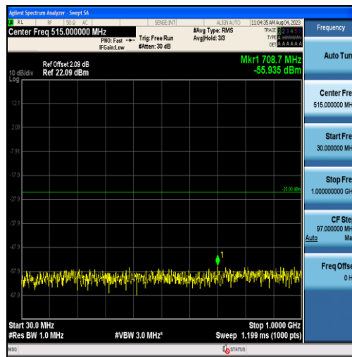
Band38-5MHz-16QAM-37775-25RB#0-Range1:30~1000MHz
