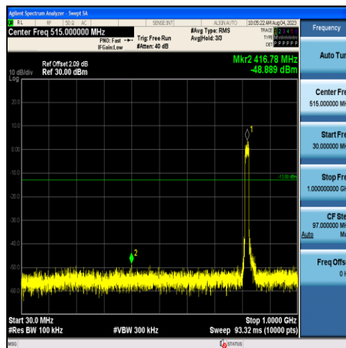
Band26-15MHz-QPSK-26765-75RB#0-Range1:30~1000MHz
