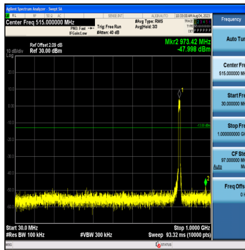
Band26-10MHz-16QAM-26990-50RB#0-Range1:30~1000MHz
