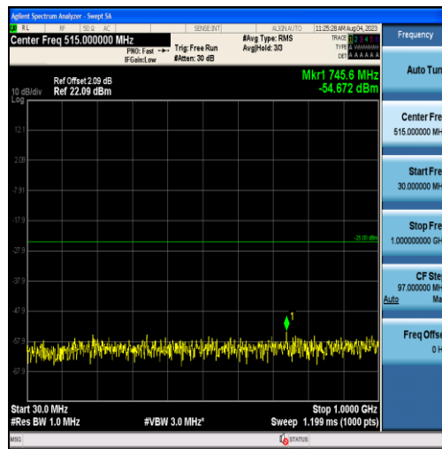
Band38-10MHz-QPSK-38000-50RB#0-Range1:30~1000MHz
