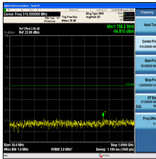
Band38-10MHz-16QAM-38000-50RB#0-Range1:30~1000MHz
