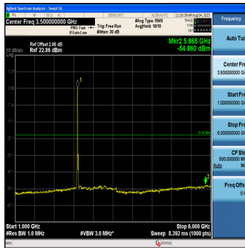
Band38-10MHz-16QAM-38000-50RB#0-Range2:1000~6000MHz
