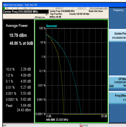
Band26-5MHz-QPSK-26740-25RB#0
