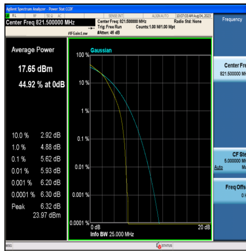
Band26-15MHz-16QAM-26765-75RB#0
