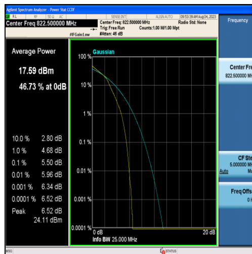
Band26-3MHz-16QAM-26775-15RB#0
