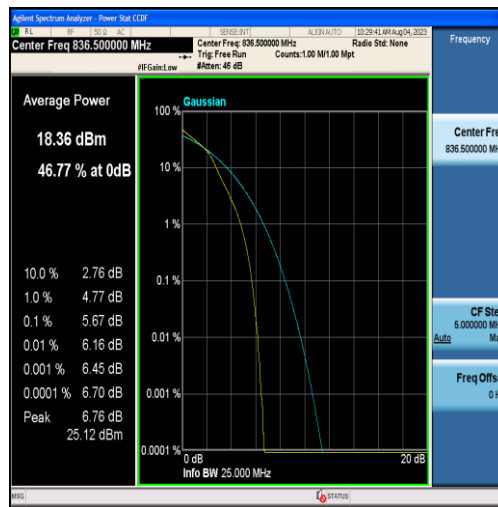
Band26-5MHz-16QAM-26915-25RB#0
