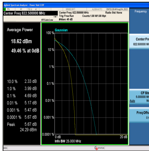
Band26-3MHz-QPSK-26775-15RB#0
