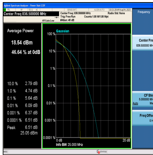
Band26-3MHz-16QAM-26915-15RB#0
