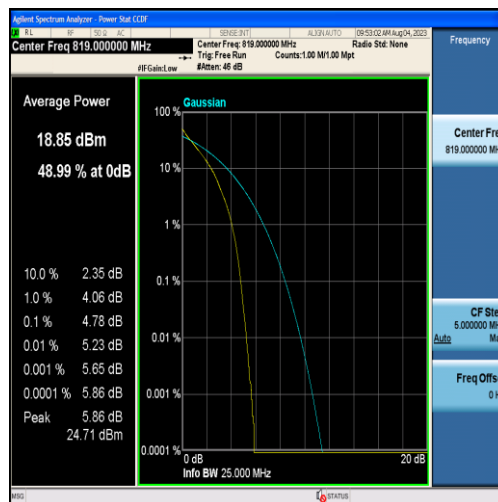
Band26-3MHz-QPSK-26740-15RB#0
