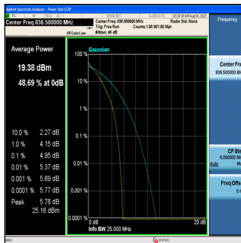
Band26-5MHz-QPSK-26915-25RB#0
