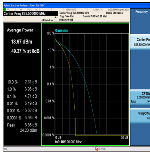
Band26-3MHz-QPSK-26805-15RB#0
