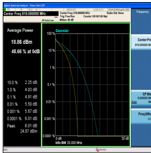
Band26-10MHz-QPSK-26740-50RB#0
