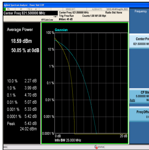
Band26-5MHz-QPSK-26765-25RB#0
