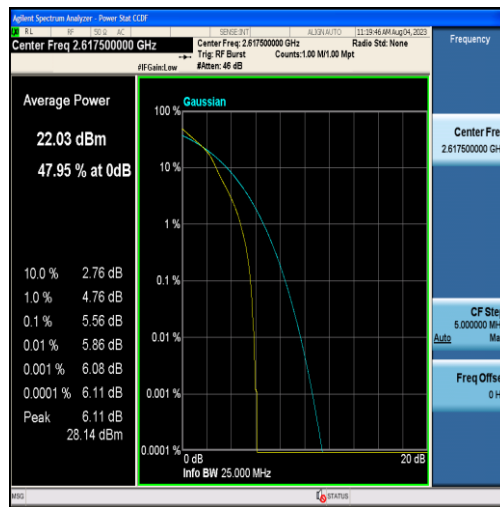
Band38-5MHz-16QAM-38225-25RB#0
