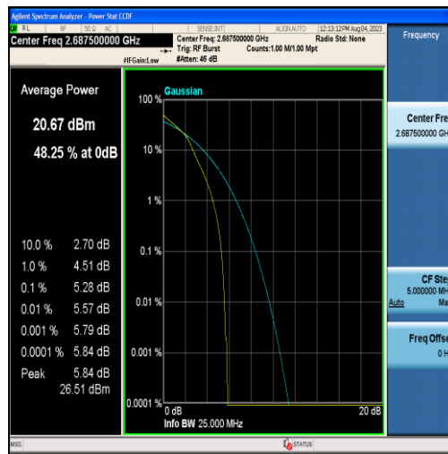
Band41-5MHz-16QAM-41565-25RB#0
