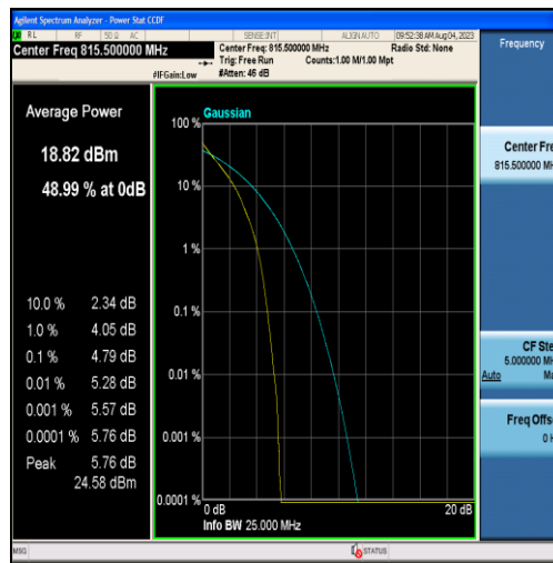
Band26-3MHz-QPSK-26705-15RB#0
