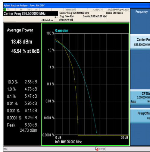
Band26-1.4MHz-16QAM-26915-6RB#0
