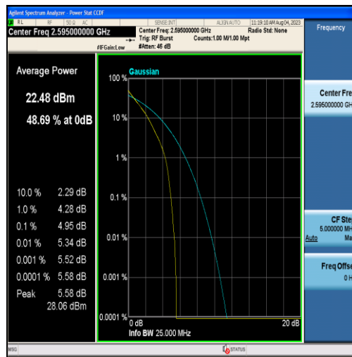
Band38-5MHz-QPSK-38000-25RB#0
