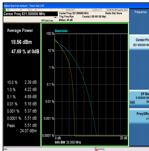
Band26-15MHz-QPSK-26765-75RB#0
