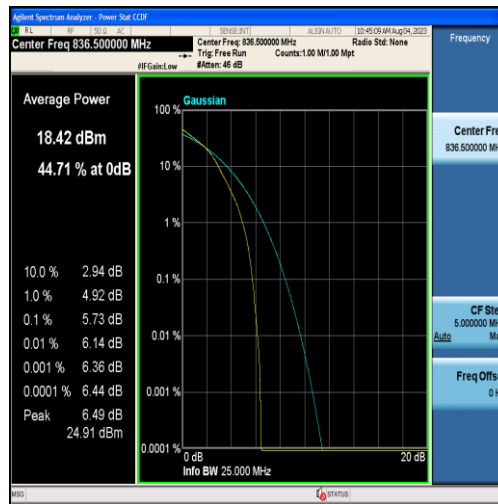
Band26-15MHz-16QAM-26915-75RB#0
