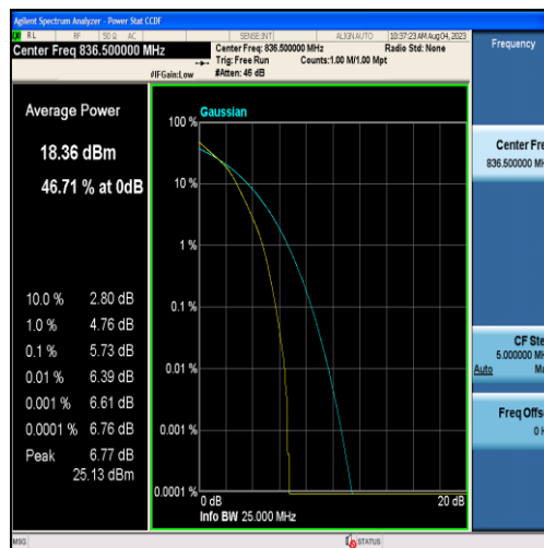
Band26-10MHz-16QAM-26915-50RB#0
