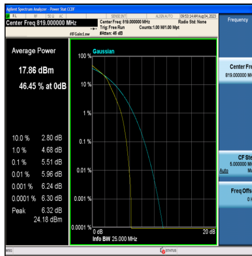
Band26-3MHz-16QAM-26740-15RB#0
