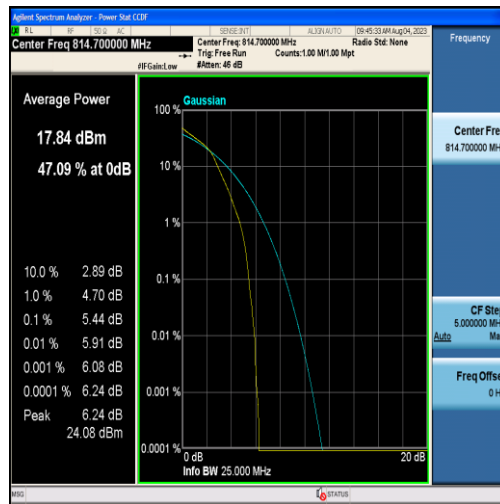
Band26-1.4MHz-16QAM-26697-6RB#0
