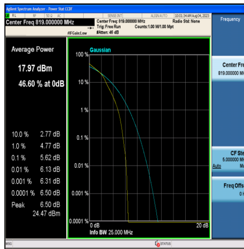
Band26-5MHz-16QAM-26740-25RB#0
