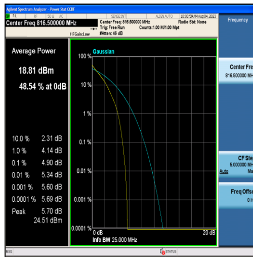
Band26-5MHz-QPSK-26715-25RB#0
