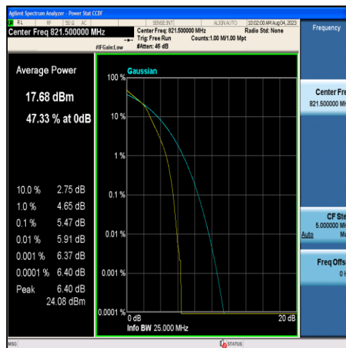
Band26-5MHz-16QAM-26765-25RB#0
