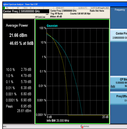
Band38-20MHz-16QAM-38000-100RB#0
