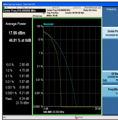
Band26-1.4MHz-16QAM-26740-6RB#0
