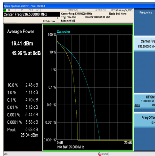
Band26-1.4MHz-QPSK-26915-6RB#0
