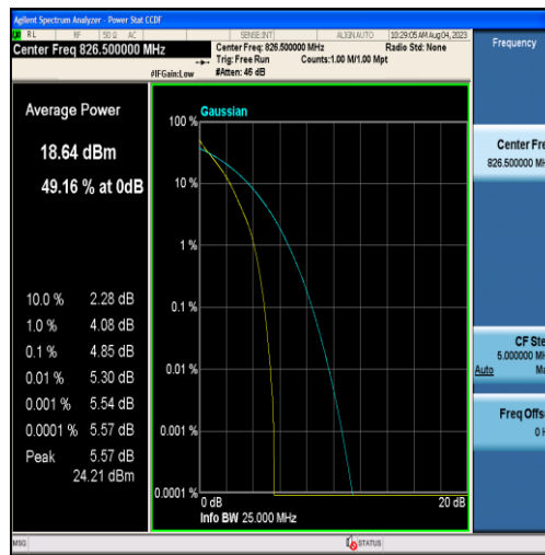
Band26-5MHz-QPSK-26815-25RB#0
