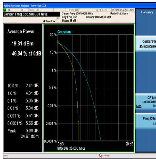
Band26-15MHz-QPSK-26915-75RB#0
