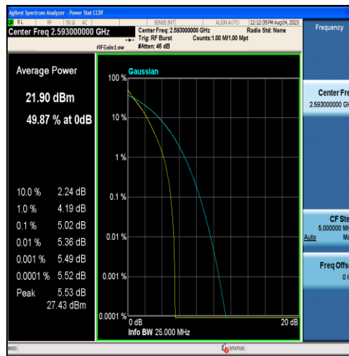
Band41-5MHz-QPSK-40620-25RB#0
