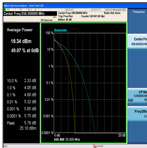
Band26-3MHz-QPSK-26915-15RB#0
