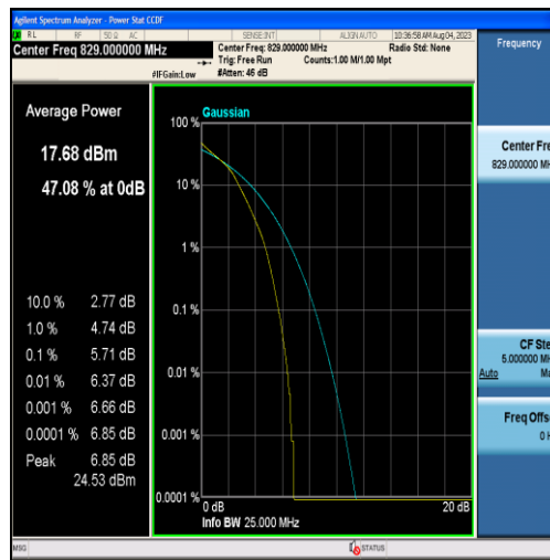
Band26-10MHz-16QAM-26840-50RB#0
