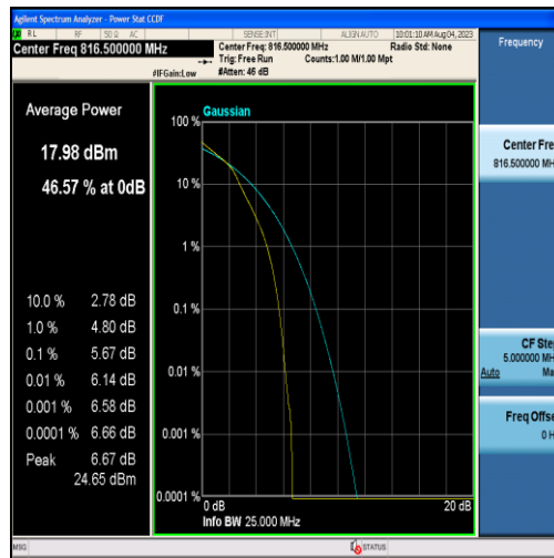
Band26-5MHz-16QAM-26715-25RB#0
