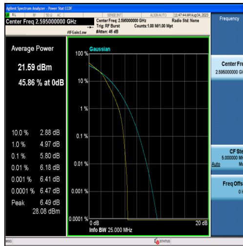
Band38-15MHz-16QAM-38000-75RB#0
