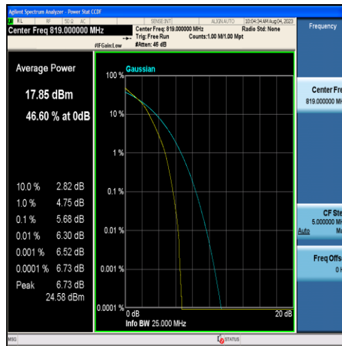
Band26-10MHz-16QAM-26740-50RB#0
