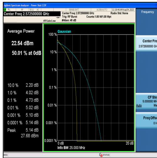
Band38-5MHz-QPSK-37775-25RB#0
