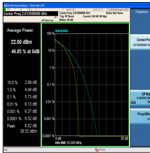
Band38-15MHz-16QAM-38175-75RB#0
