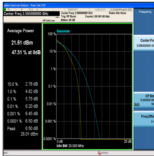
Band38-10MHz-16QAM-38000-50RB#0
