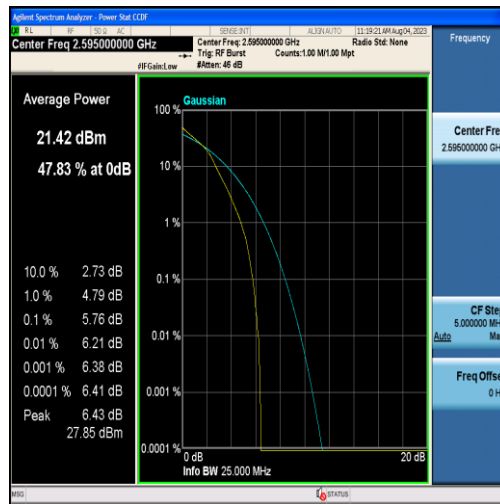
Band38-5MHz-16QAM-38000-25RB#0
