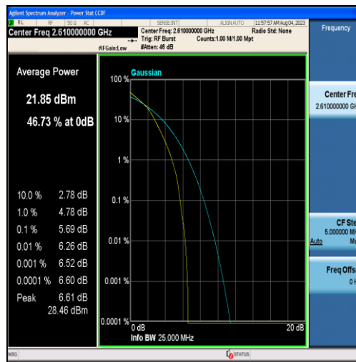
Band38-20MHz-16QAM-38150-100RB#0
