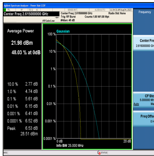
Band38-10MHz-16QAM-38200-50RB#0
