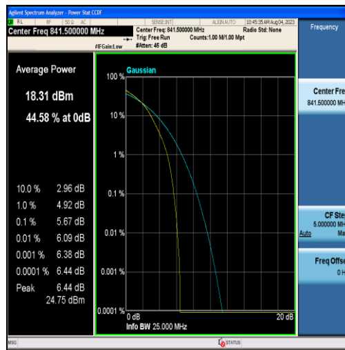
Band26-15MHz-16QAM-26965-75RB#0
