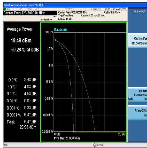
Band26-1.4MHz-QPSK-26783-6RB#0
