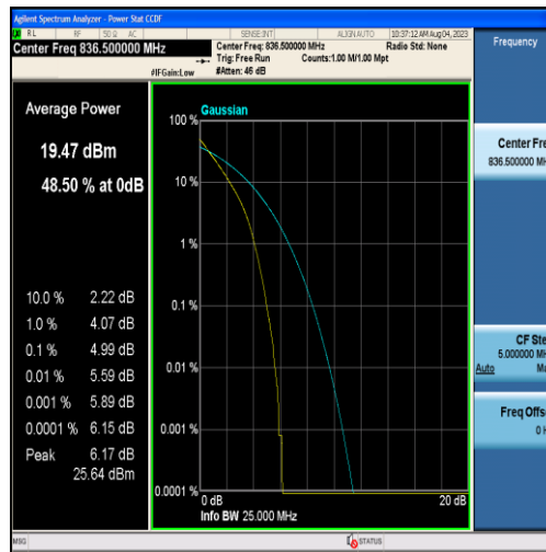
Band26-10MHz-QPSK-26915-50RB#0
