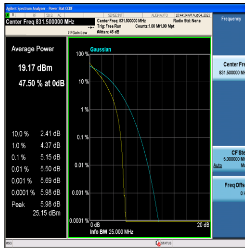
Band26-15MHz-QPSK-26865-75RB#0
