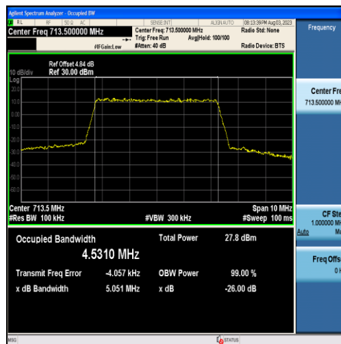
Band12-5MHz-QPSK-23155-25RB#0-4.5310
