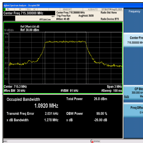
Band12-1.4MHz-QPSK-23173-6RB#0-1.0920
