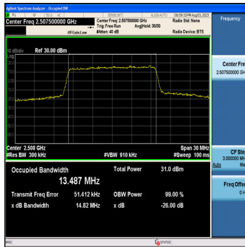
Band7-15MHz-QPSK-20825-75RB#0-13.487
