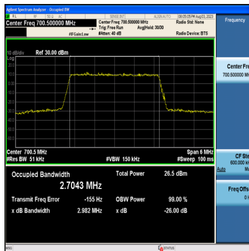
Band12-3MHz-16QAM-23025-15RB#0-2.7043
