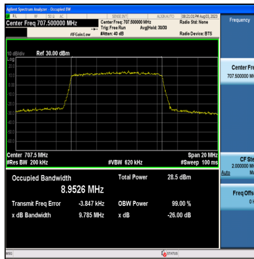
Band12-10MHz-QPSK-23095-50RB#0-8.9526
