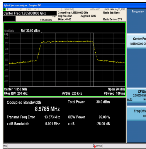
Band25-10MHz-QPSK-26090-50RB#0-8.9785
