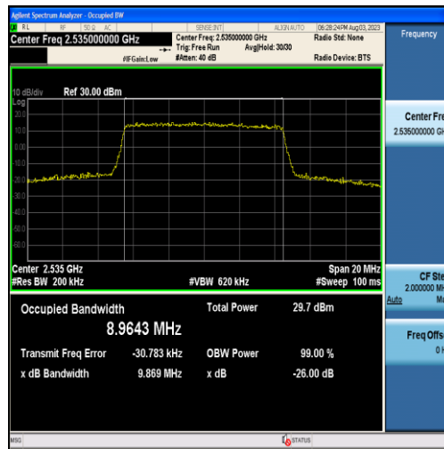
Band7-10MHz-16QAM-21100-50RB#0-8.9643
