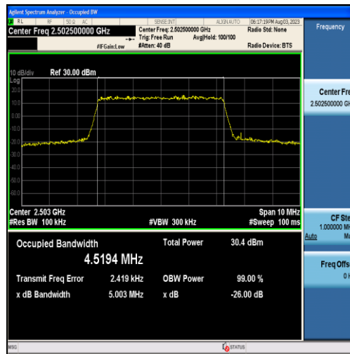
Band7-5MHz-QPSK-20775-25RB#0-4.5194
