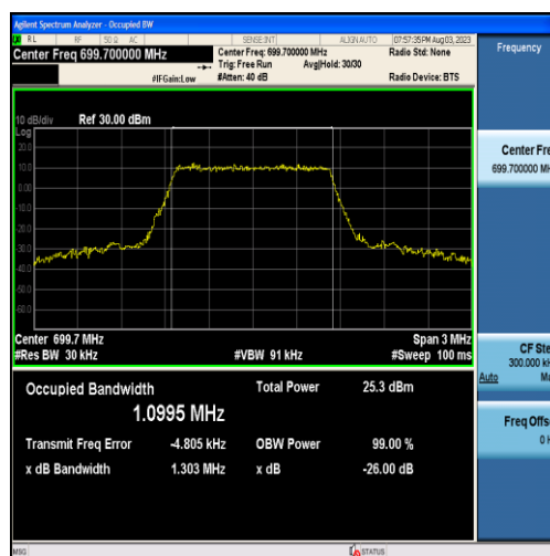
Band12-1.4MHz-16QAM-23017-6RB#0-1.0995
