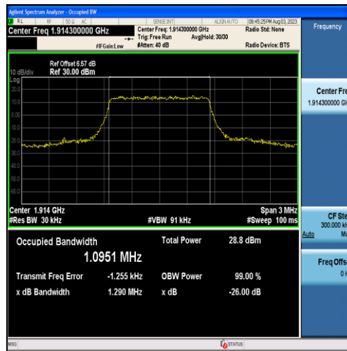
Band25-1.4MHz-QPSK-26683-6RB#0-1.0951
