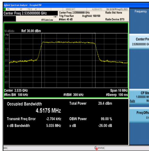
Band7-5MHz-16QAM-21100-25RB#0-4.5175
