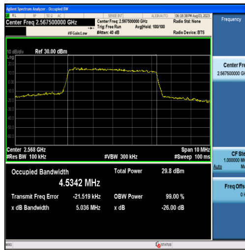
Band7-5MHz-16QAM-21425-25RB#0-4.5342
