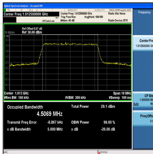
Band25-5MHz-16QAM-26665-25RB#0-4.5069
