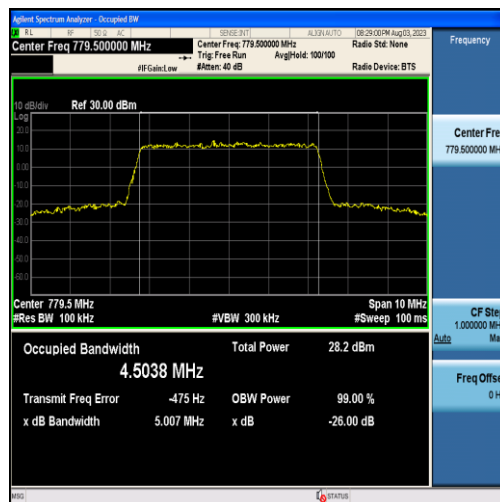
Band13-5MHz-16QAM-23205-25RB#0-4.5038
