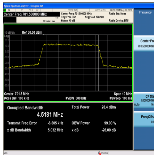
Band12-5MHz-QPSK-23035-25RB#0-4.5181
