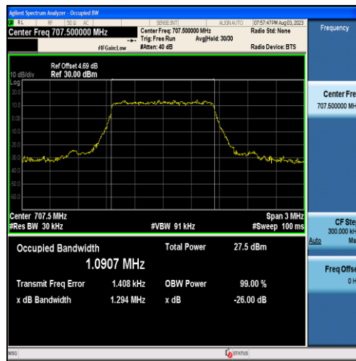
Band12-1.4MHz-QPSK-23095-6RB#0-1.0907
