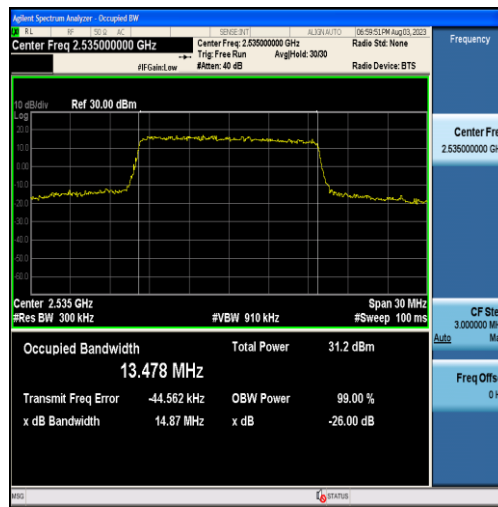
Band7-15MHz-QPSK-21100-75RB#0-13.478
