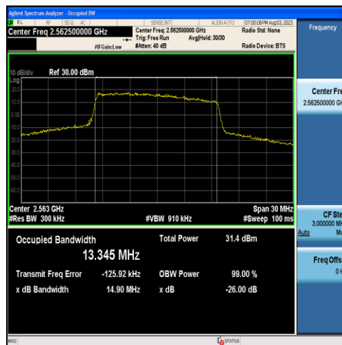
Band7-15MHz-QPSK-21375-75RB#0-13.345
