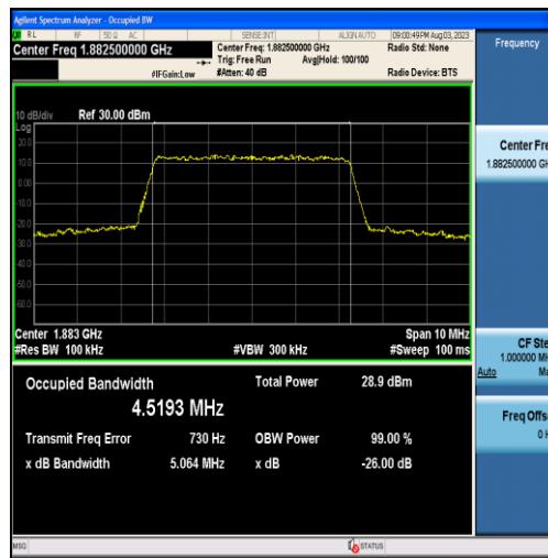
Band25-5MHz-16QAM-26365-25RB#0-4.5193
