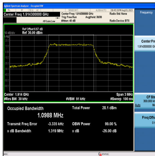
Band25-1.4MHz-16QAM-26683-6RB#0-1.0988
