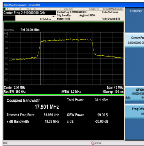
Band7-20MHz-QPSK-20850-100RB#0-17.901
