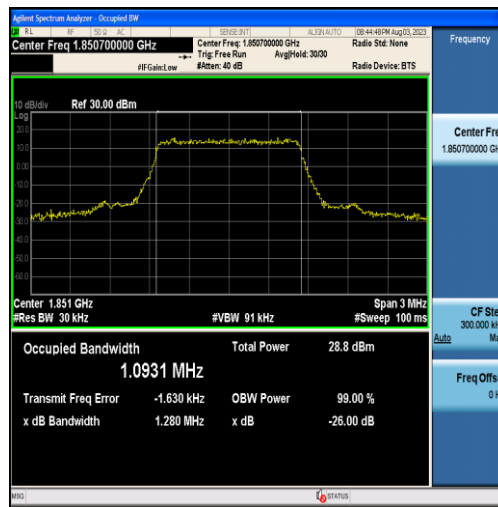
Band25-1.4MHz-QPSK-26047-6RB#0-1.0931
