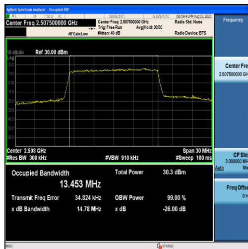
Band7-15MHz-16QAM-20825-75RB#0-13.453
