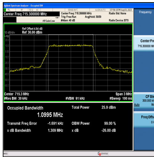
Band12-1.4MHz-16QAM-23173-6RB#0-1.0995
