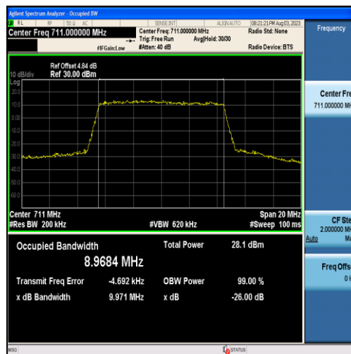
Band12-10MHz-QPSK-23130-50RB#0-8.9684
