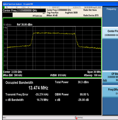
Band7-15MHz-16QAM-21100-75RB#0-13.474
