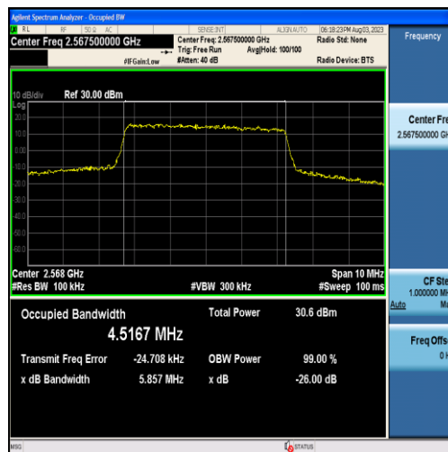
Band7-5MHz-QPSK-21425-25RB#0-4.5167
