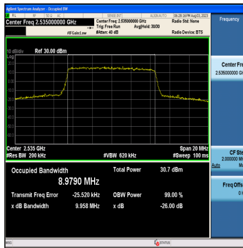
Band7-10MHz-QPSK-21100-50RB#0-8.9790
