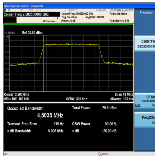
Band7-5MHz-16QAM-20775-25RB#0-4.5035
