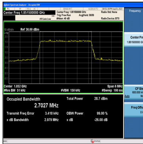
Band25-3MHz-16QAM-26055-15RB#0-2.7027
