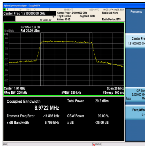
Band25-10MHz-16QAM-26640-50RB#0-8.9722
