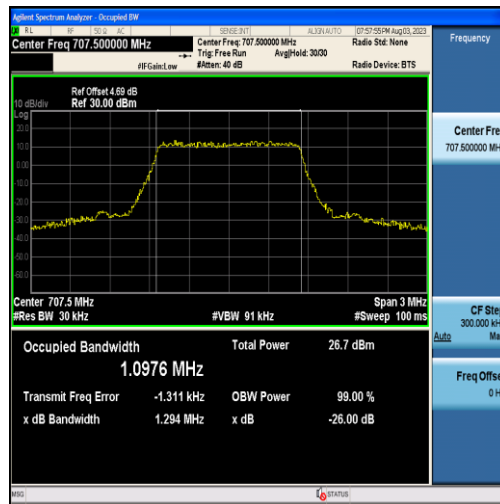
Band12-1.4MHz-16QAM-23095-6RB#0-1.0976
