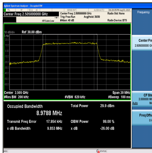
Band7-10MHz-16QAM-20800-50RB#0-8.9788
