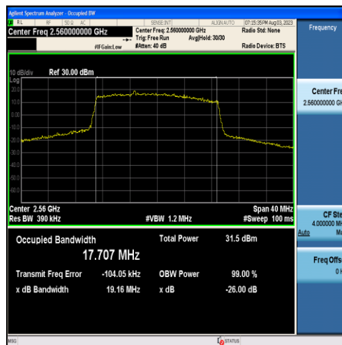
Band7-20MHz-QPSK-21350-100RB#0-17.707
