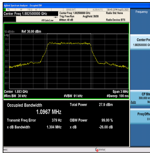
Band25-1.4MHz-16QAM-26365-6RB#0-1.0967
