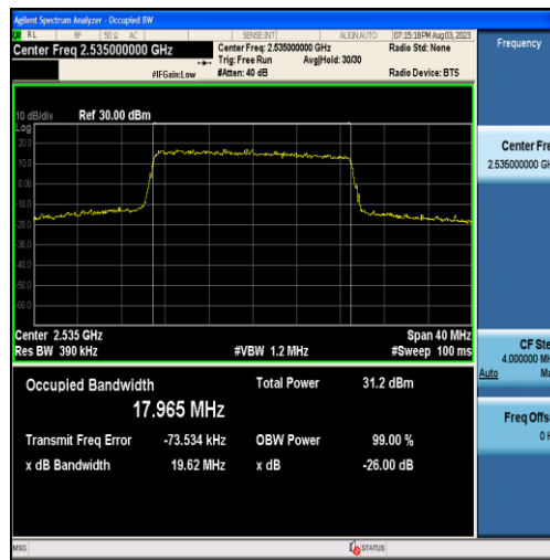
Band7-20MHz-QPSK-21100-100RB#0-17.965
