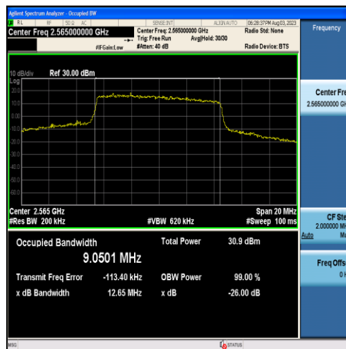
Band7-10MHz-QPSK-21400-50RB#0-9.0501
