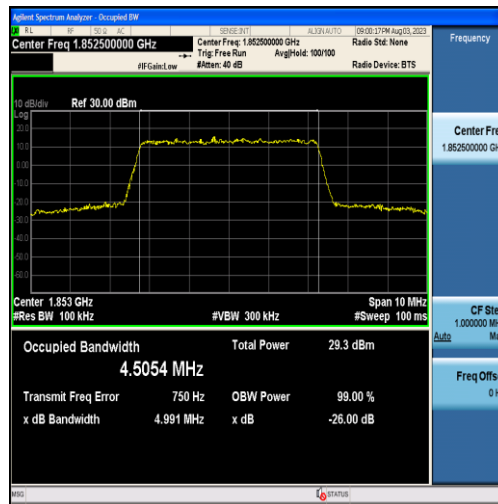
Band25-5MHz-16QAM-26065-25RB#0-4.5054
