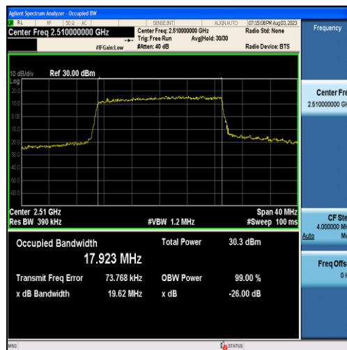
Band7-20MHz-16QAM-20850-100RB#0-17.923
