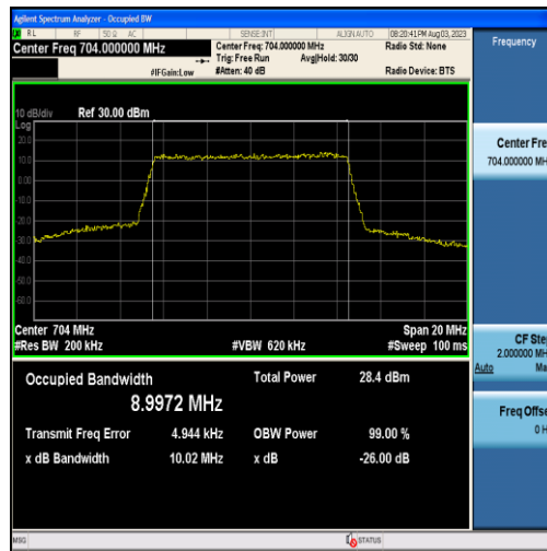
Band12-10MHz-QPSK-23060-50RB#0-8.9972
