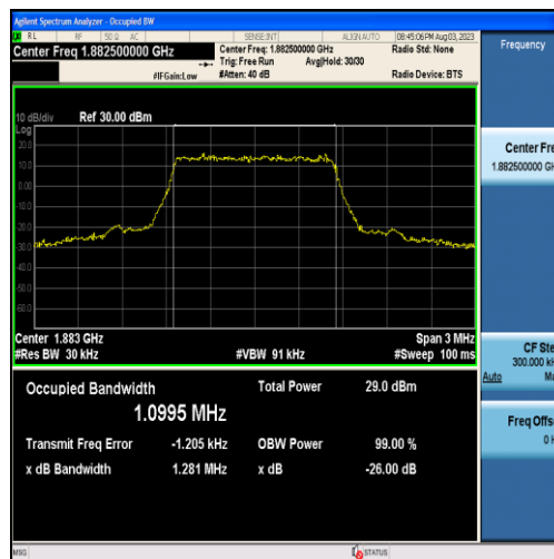
Band25-1.4MHz-QPSK-26365-6RB#0-1.0995
