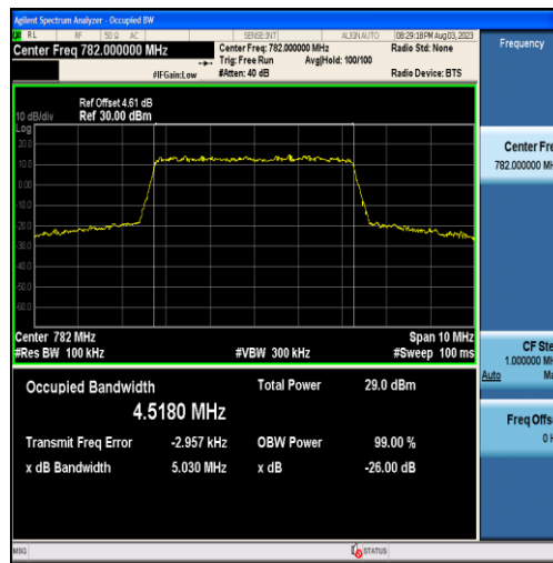
Band13-5MHz-QPSK-23230-25RB#0-4.5180
