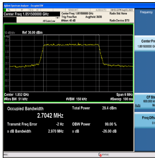
Band25-3MHz-QPSK-26055-15RB#0-2.7042
