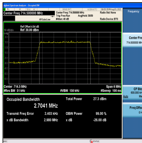
Band12-3MHz-QPSK-23165-15RB#0-2.7041
