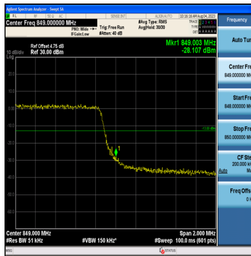
Band26-3MHz-16QAM-27025-15RB#0
