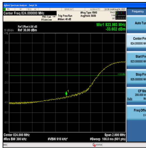
Band26-15MHz-16QAM-26865-75RB#0
