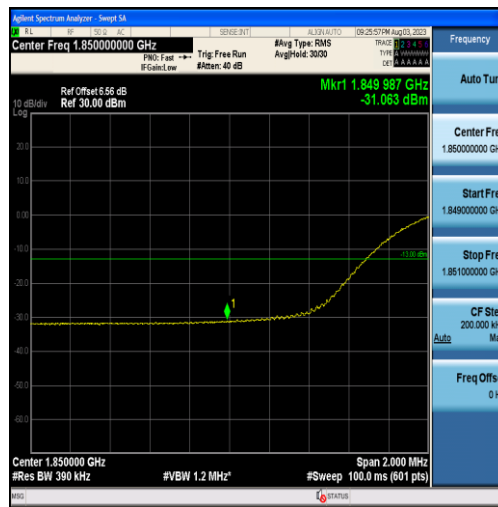
Band25-20MHz-16QAM-26140-100RB#0
