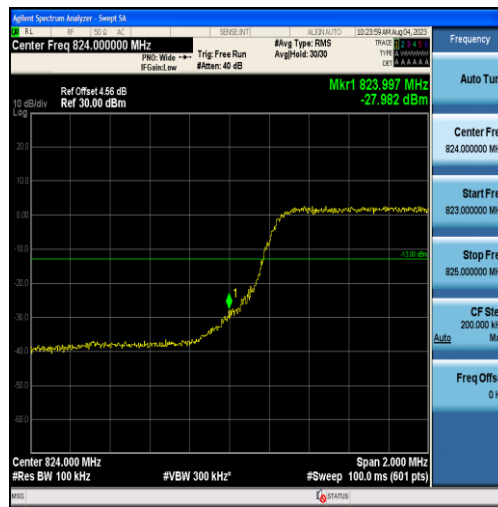
Band26-5MHz-16QAM-26815-25RB#0
