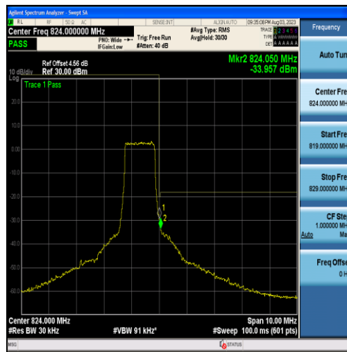
Band26-1.4MHz-16QAM-26783-6RB#0
