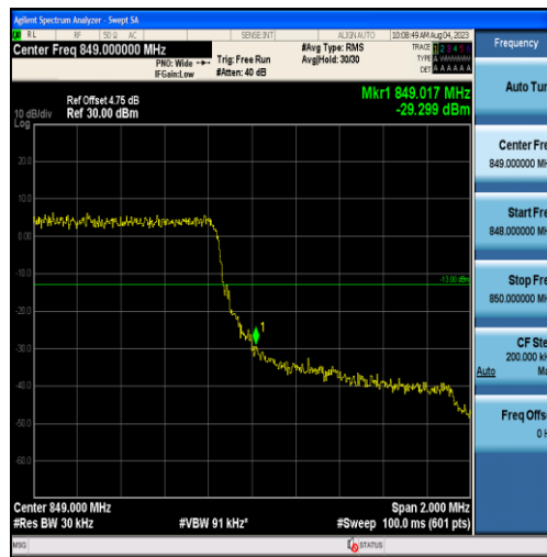
Band26-1.4MHz-QPSK-27033-6RB#0
