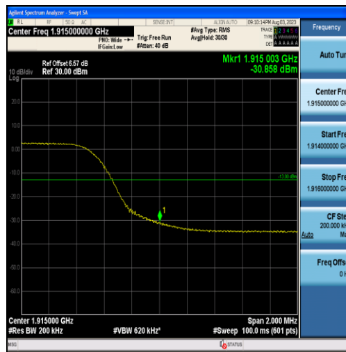
Band25-10MHz-16QAM-26640-50RB#0
