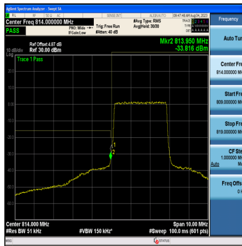
Band26-3MHz-16QAM-26705-15RB#0
