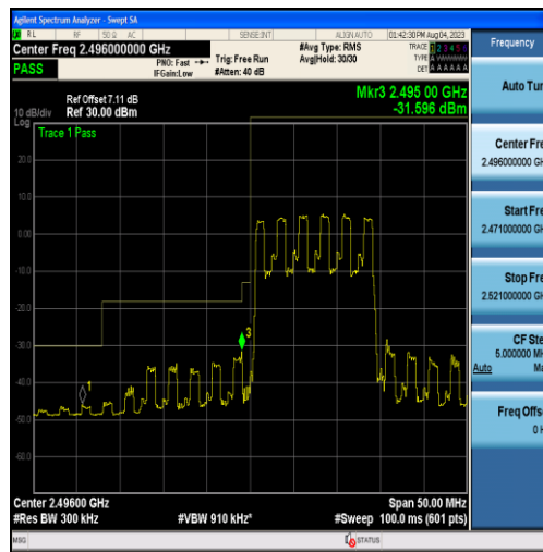
Band41-15MHz-QPSK-39725-75RB#0
