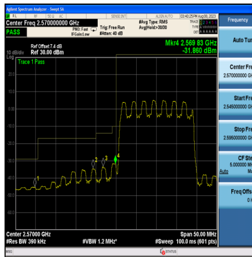
Band38-20MHz-QPSK-37850-100RB#0
