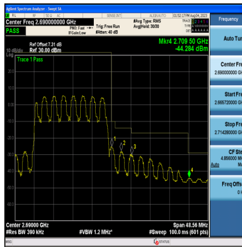
Band41-20MHz-QPSK-41490-100RB#0
