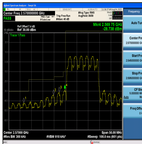
Band38-15MHz-QPSK-37825-75RB#0
