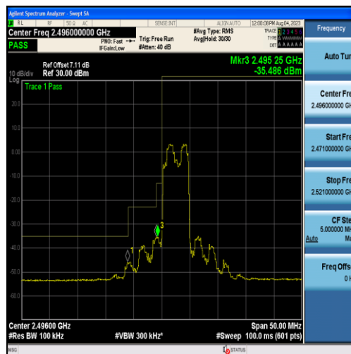
Band41-5MHz-16QAM-39675-25RB#0
