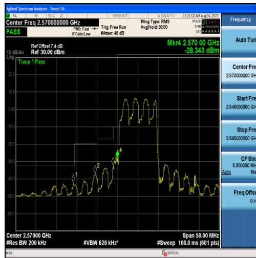
Band38-10MHz-QPSK-37800-50RB#0
