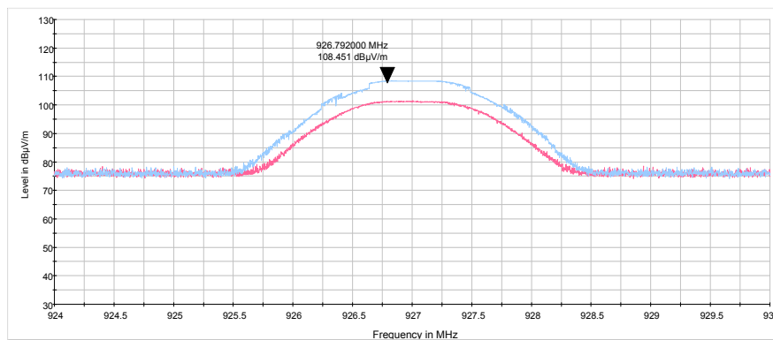
Plot 7.2.10 Field strength of carrier at high frequency
