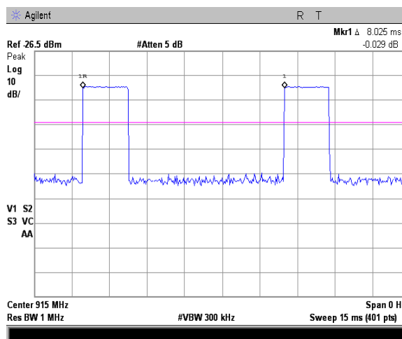
Plot 7.3.25 Transmission pulse period
