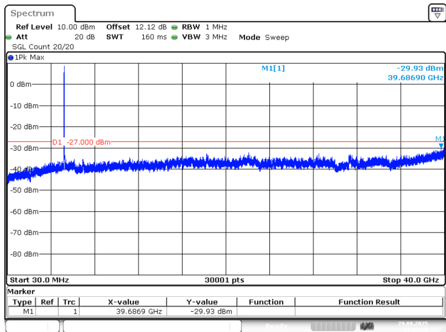
Tx. Spurious NVNT ax40 5230MHz Ant2 Emission
