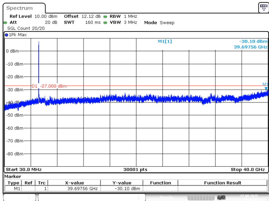
Tx. Spurious NVNT ax40 5230MHz Ant4 Emission
