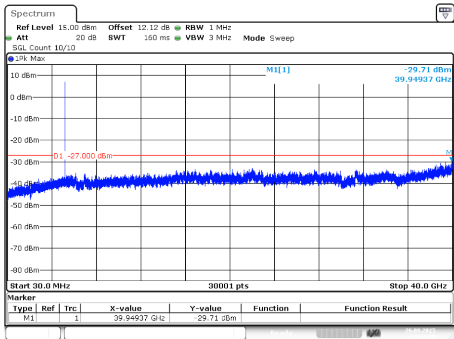
Tx. Spurious NVNT ac20 5180MHz Ant4 Emission
