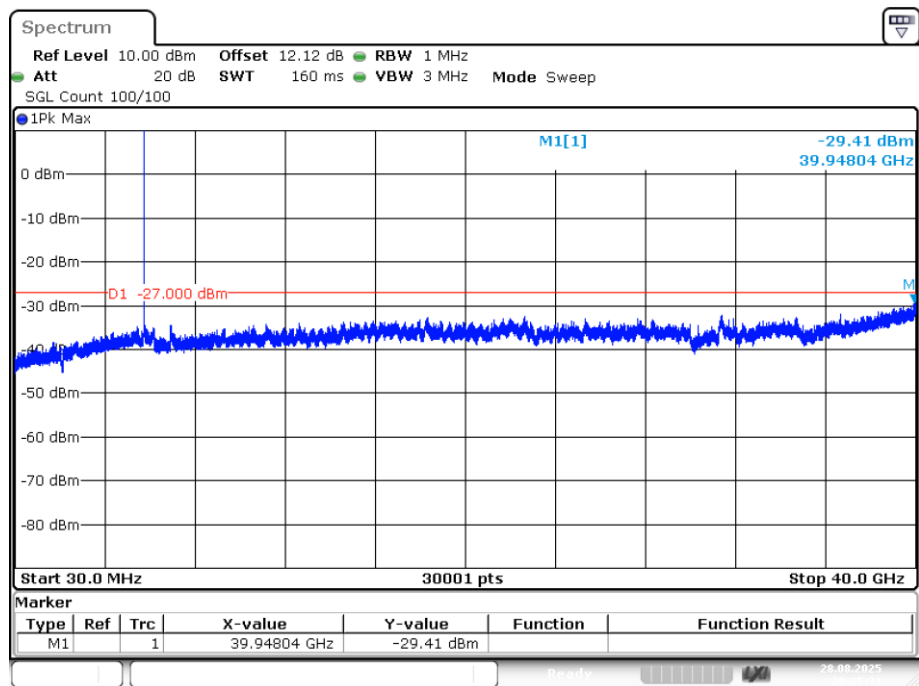
Tx. Spurious NVNT ax20 5745MHz Ant2 Emission
