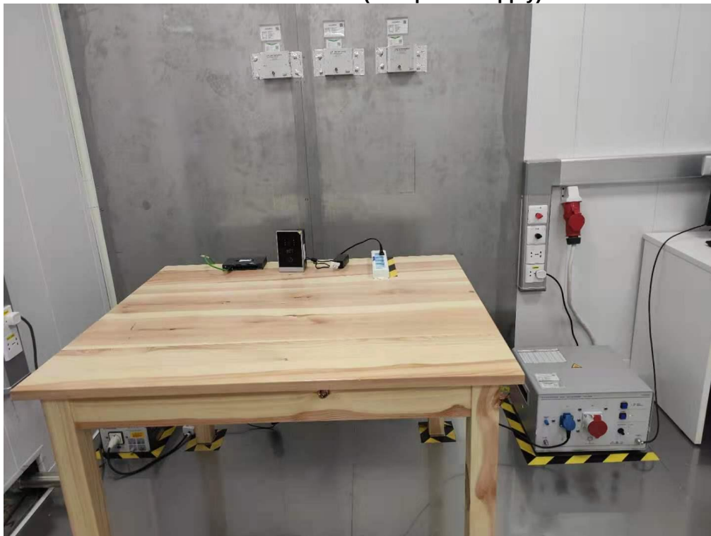
Conducted Emission(POE power supply)
