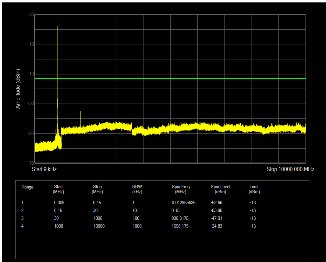
Band5 BPSK Channel=20401 nTones=1@0 Spacing=3.75kHz
