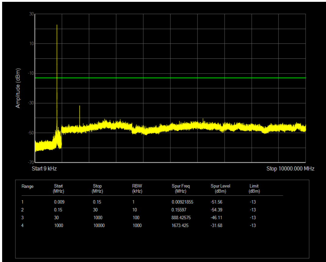
Band5 QPSK Channel=20525 nTones=1@47 Spacing=3.75kHz
