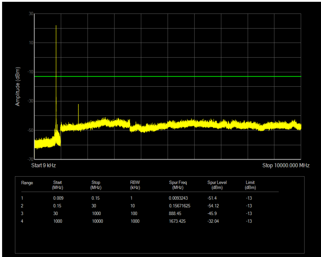
Band5 QPSK Channel=20649 nTones=1@0 Spacing=15kHz
