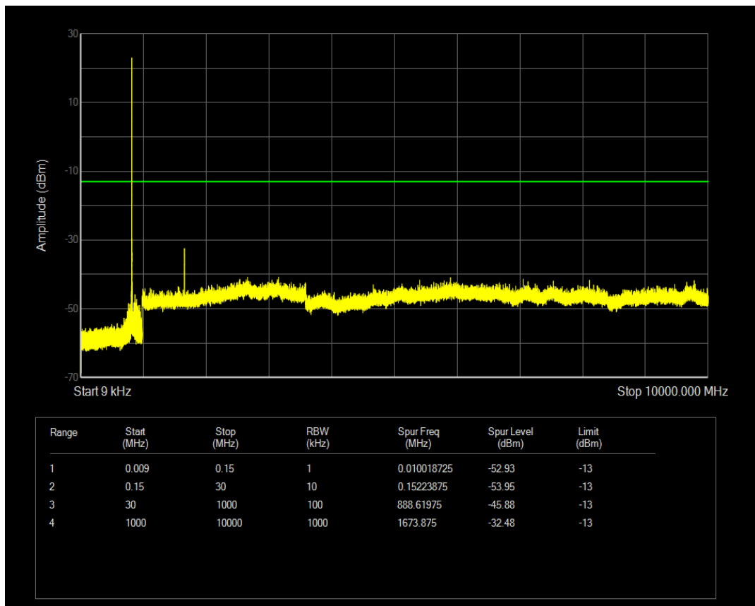
Band5 BPSK Channel=20649 nTones=1@0 Spacing=3.75kHz
