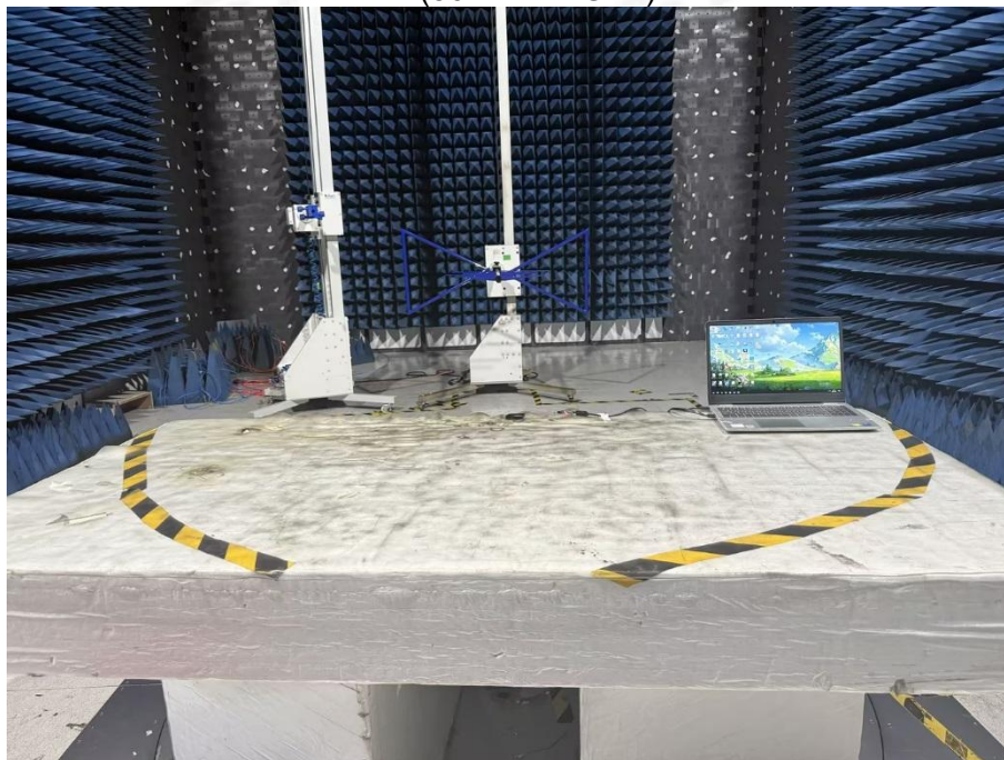
RE (30MHz - 1GHz)
