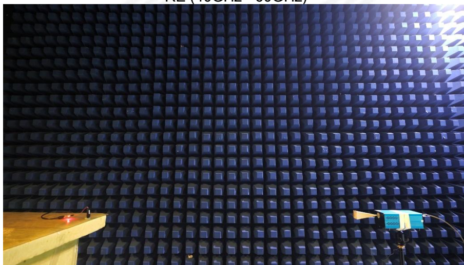
RE (40GHz - 60GHz)
