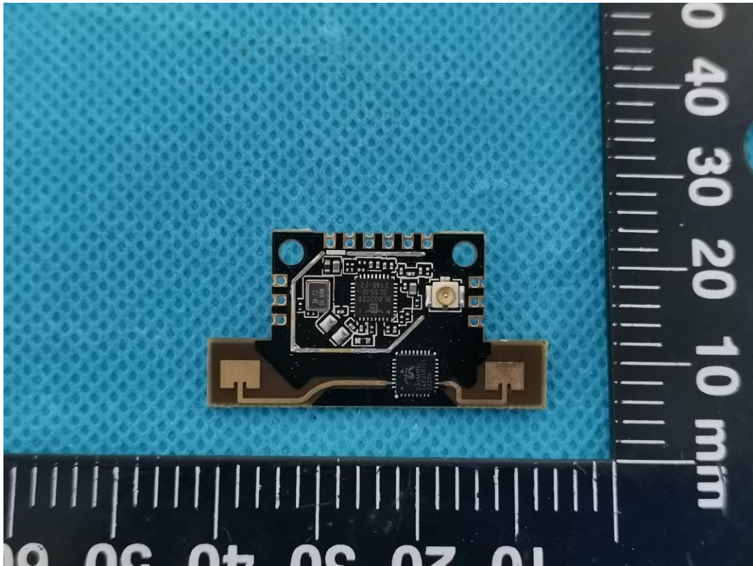
BT&WIFI chip
