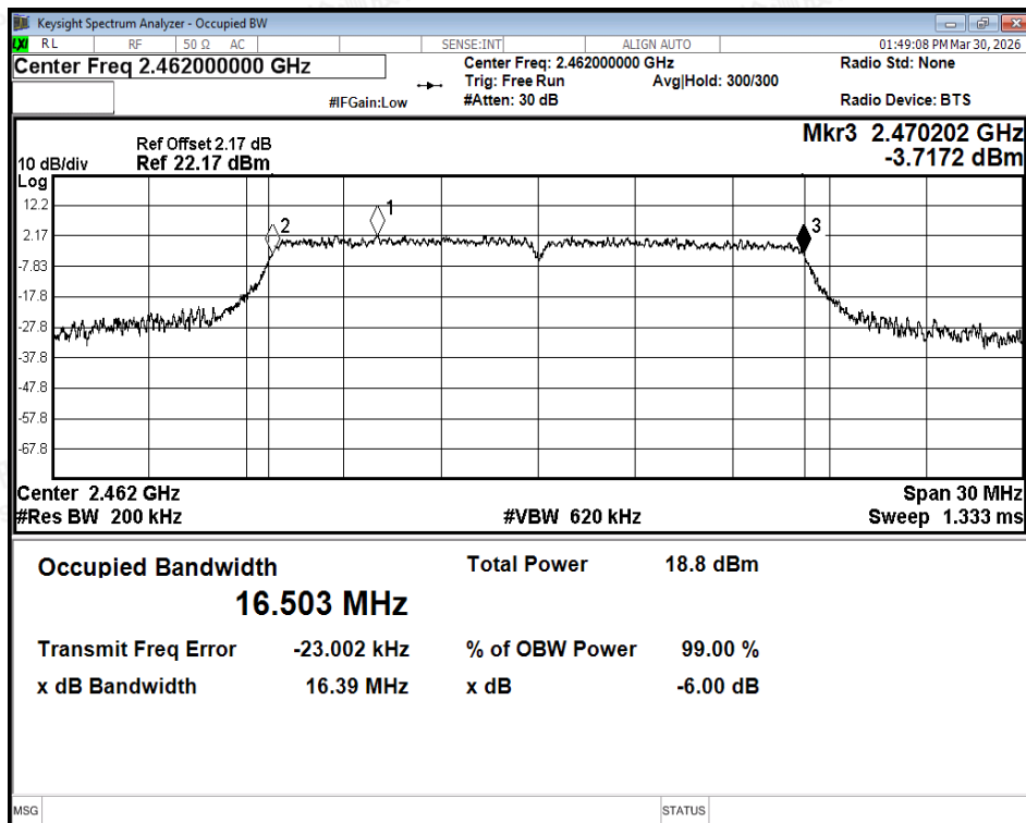
-6dB Bandwidth NVNT g 2462MHz Ant2
