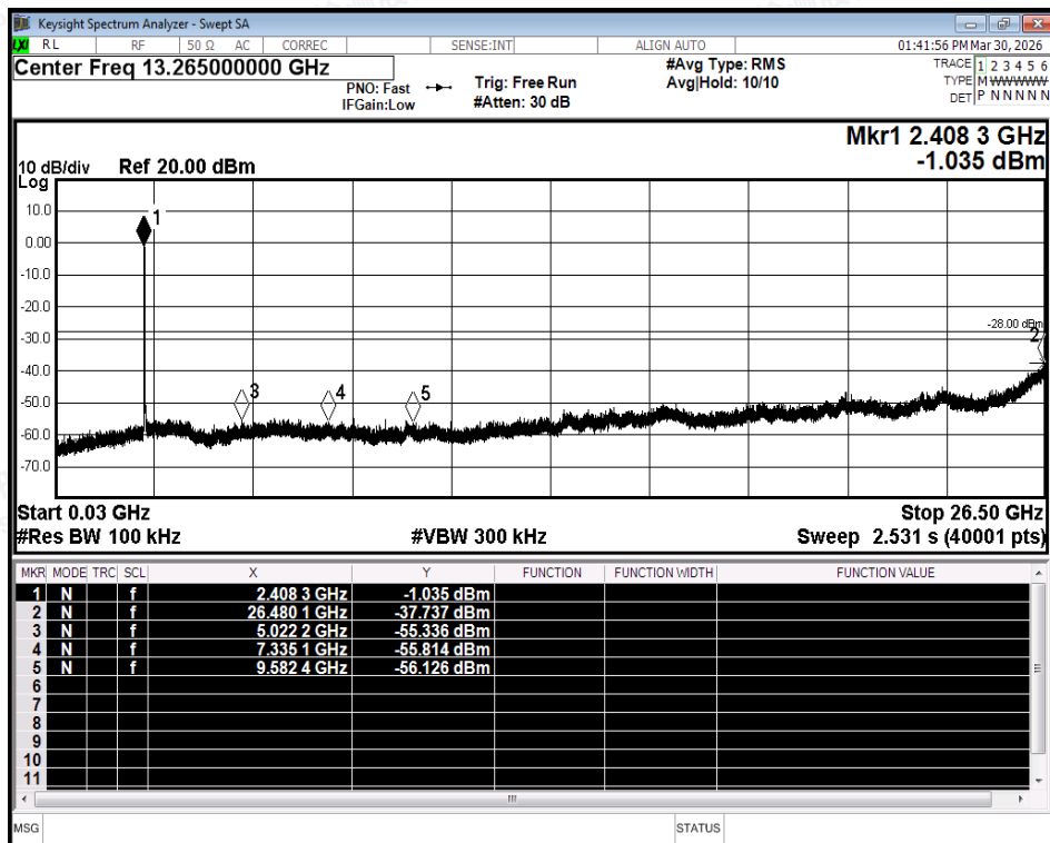
Tx. Spurious NVNT g 2412MHz Ant2 Emission
