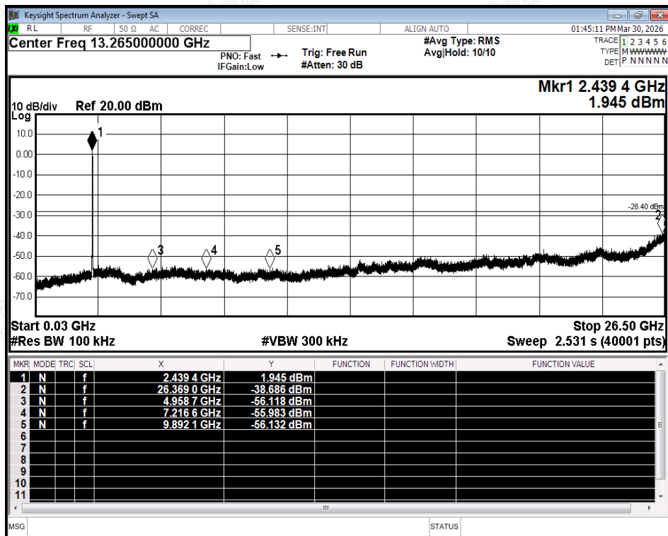
Tx. Spurious NVNT g 2437MHz Ant2 Emission
