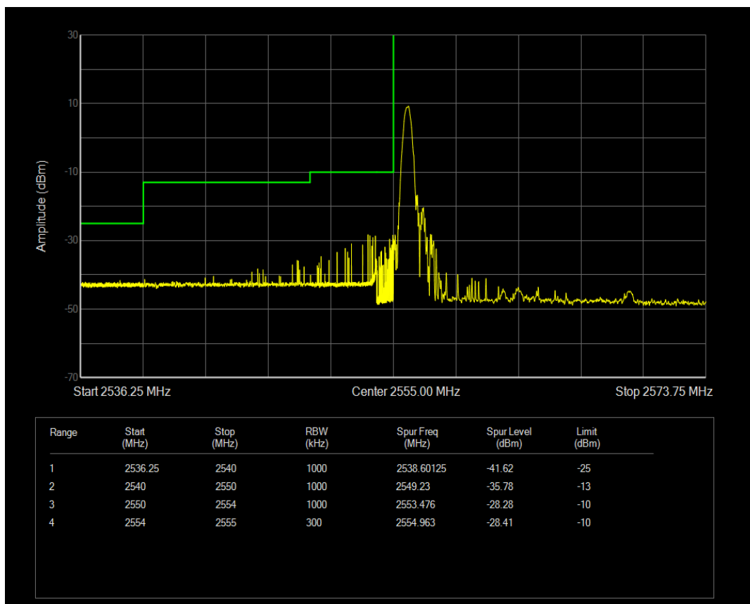
LTE Band41 QPSK BW=15MHz Channel=40315 RB Size=1 Position=#0
