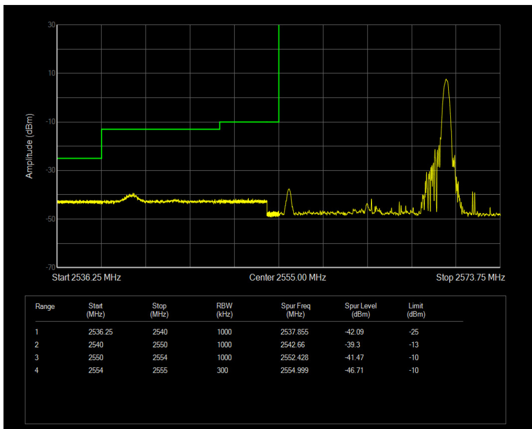
LTE Band41 QAM16 BW=15MHz Channel=40315 RB Size=1 Position=#Max
