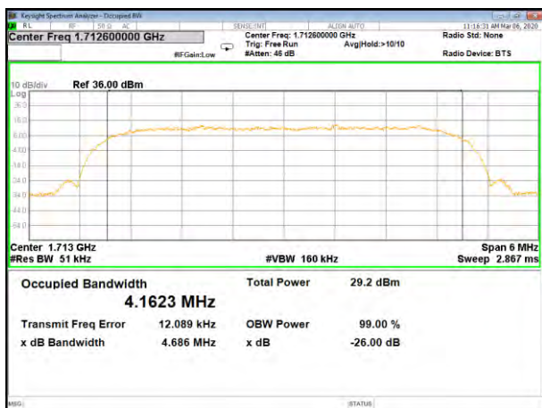
B4_WCDMA_Lower_26BW and 99%
