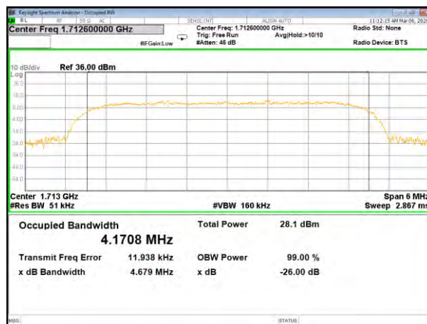
B4_HSDPA_Lower_26BW and 99%
