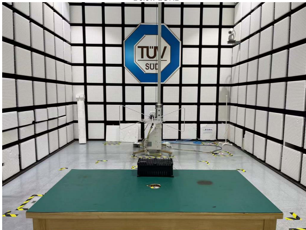
Below 1GHz
