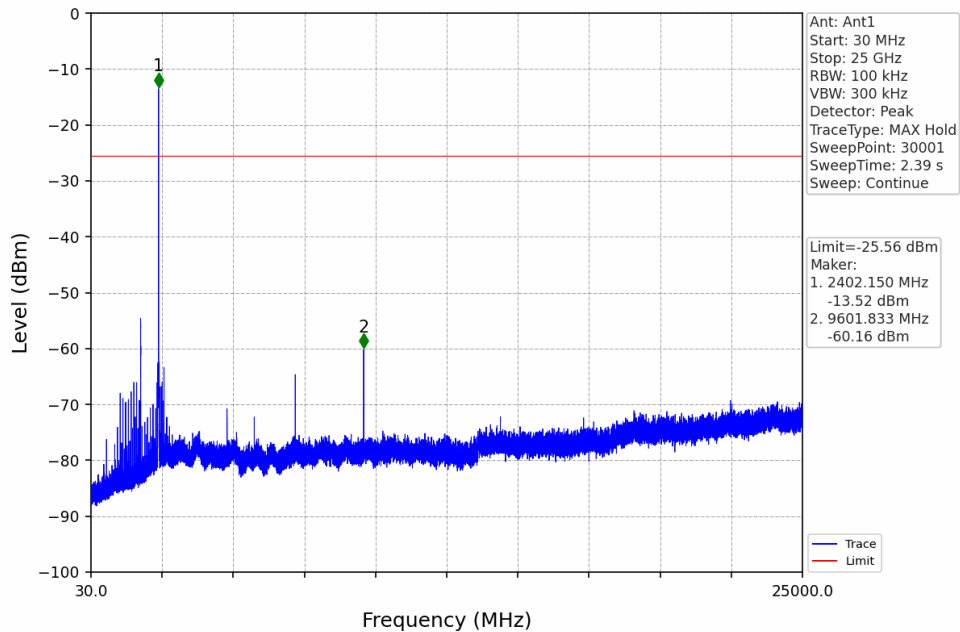
8DPSK_3DH5_LCH_2402MHz_Ant1_NTNV
