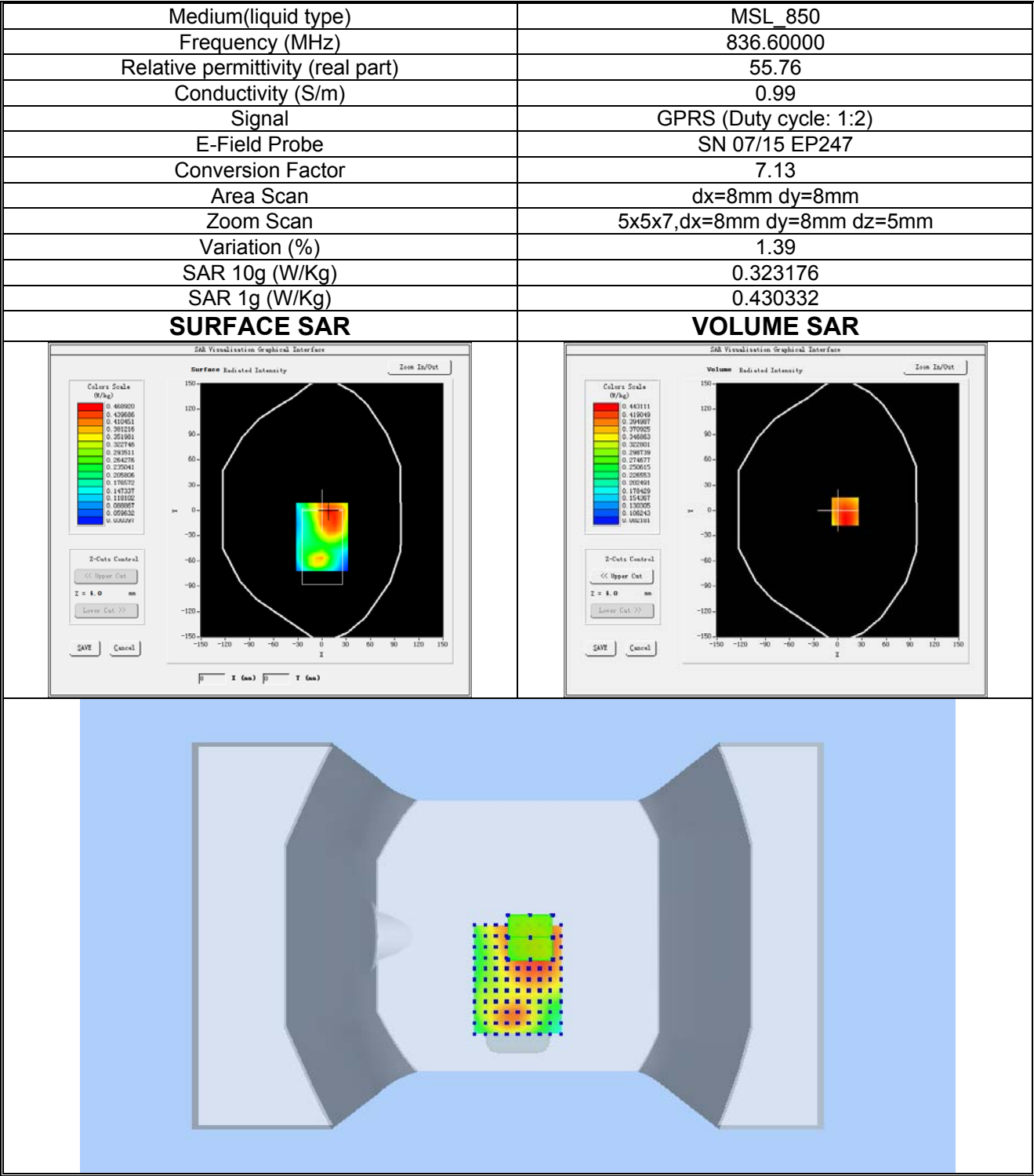
Plot 2: GPRS850MHz, Middle channel (Body-worn/Hotspot, Back Surface) Product Description:Smartphone Test Date: 2019-05-15
