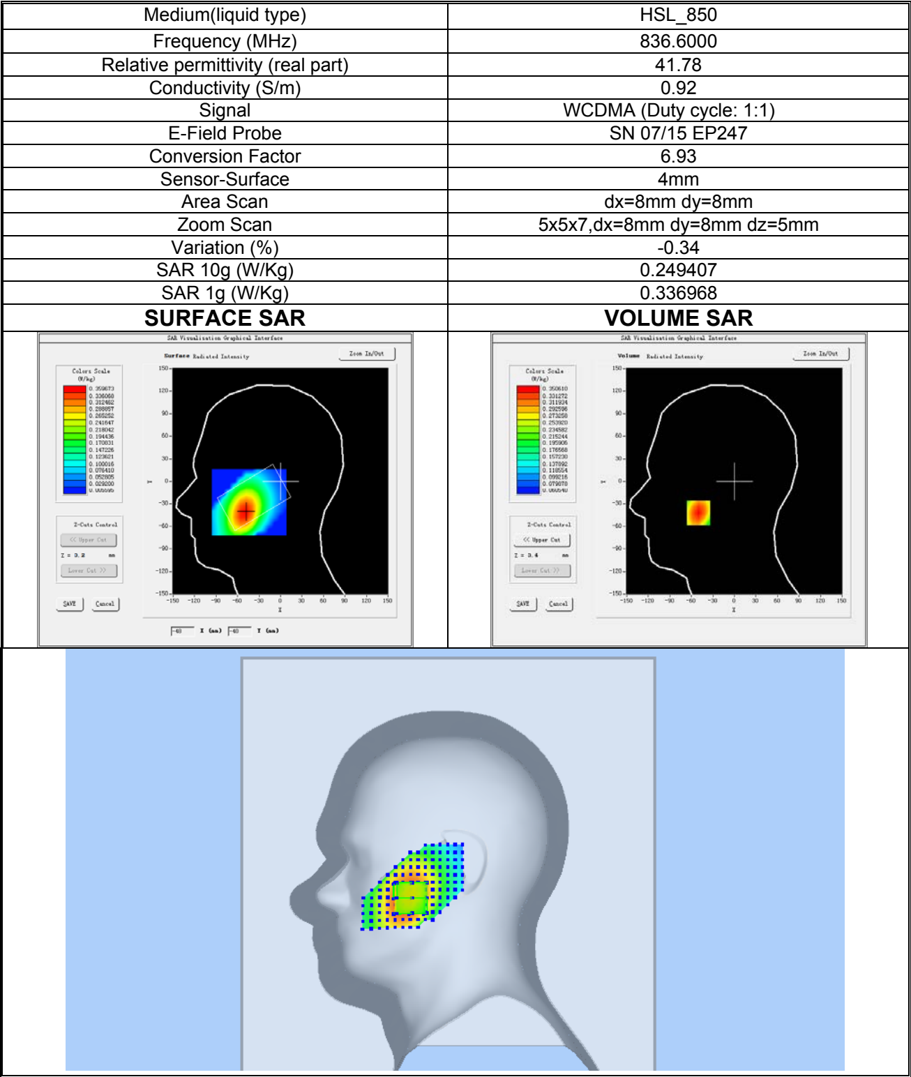
Plot 5: WCDMA BAND V, Middle channel (Right Head Cheek) Product Description: Smartphone Test Date: 2019-05-15
