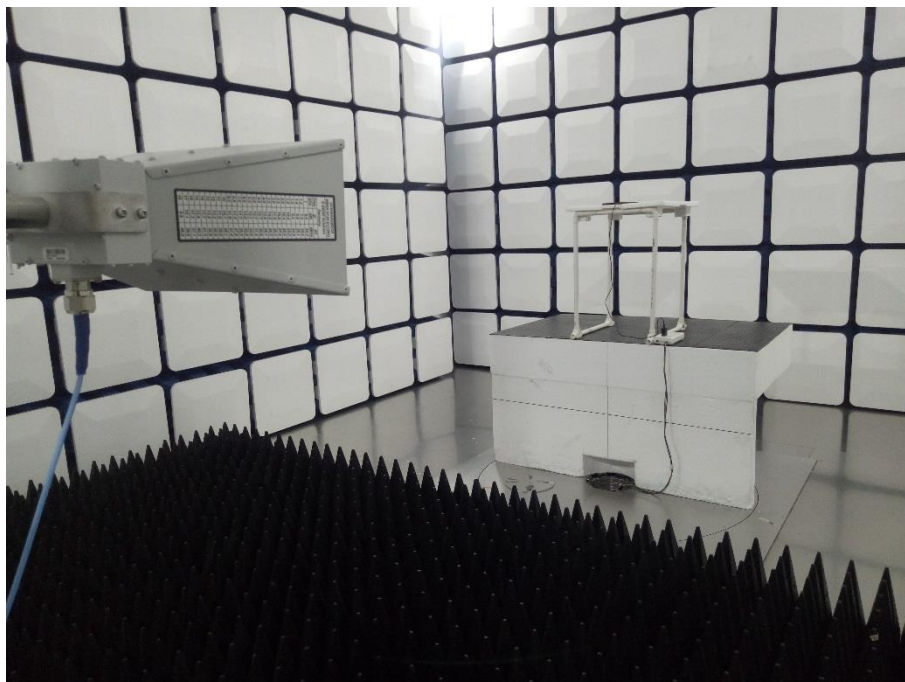
Above 1GHz (8 inches)
