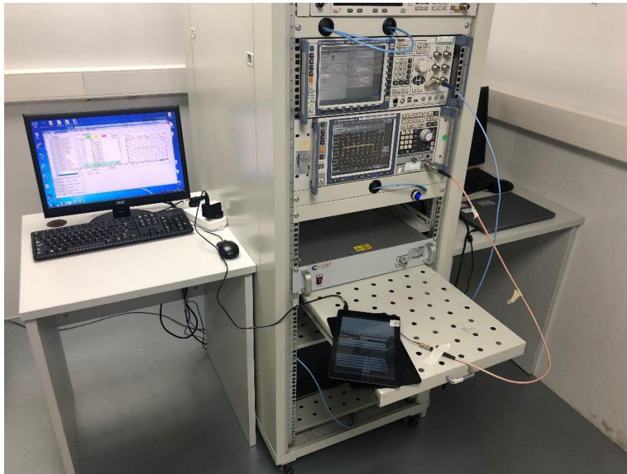
Conducted Test-WIFI (10 inches)
