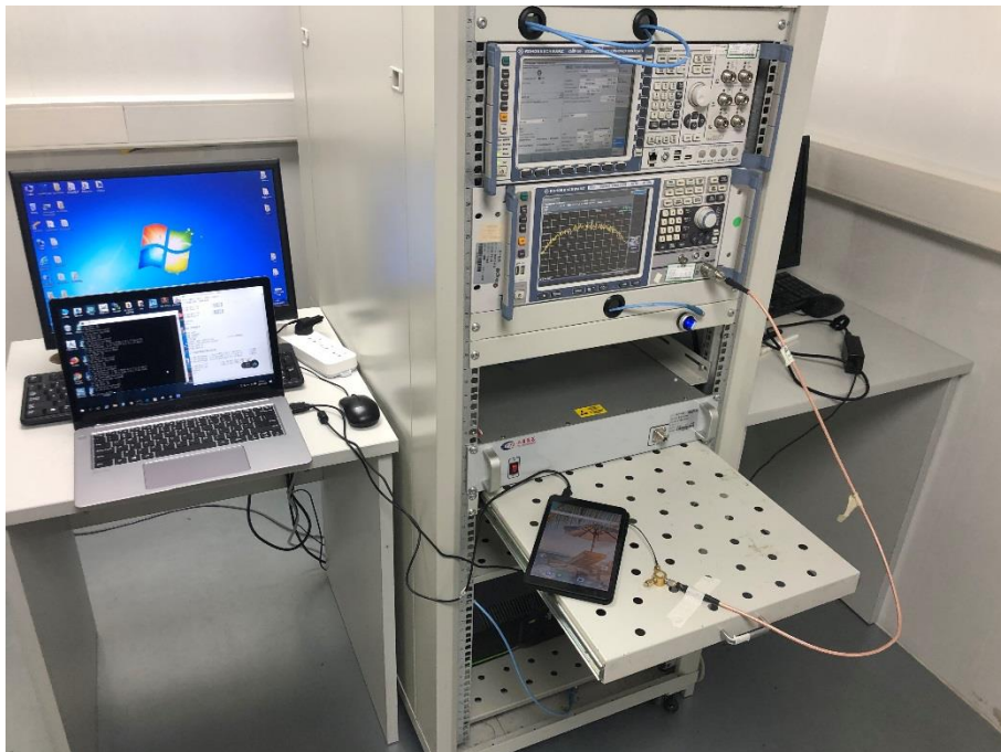
Conducted Test-BT (8 inches)
