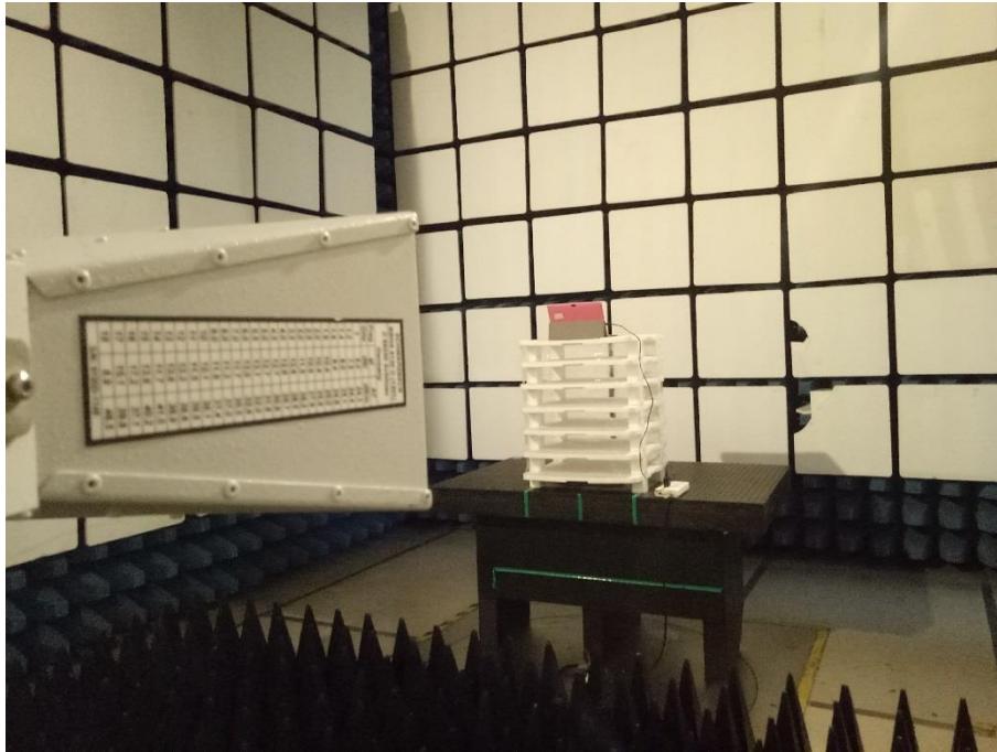
Above 1GHz (10 inches)
