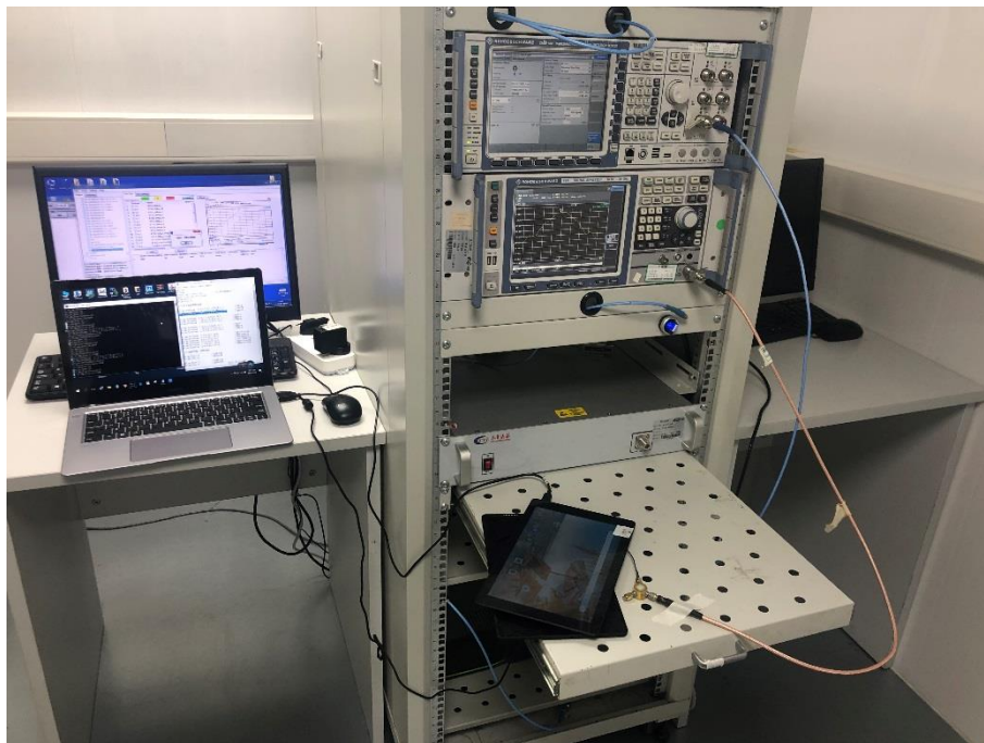
Conducted Test-BLE (10 inches)
