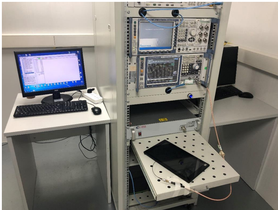
Conducted Test-WIFI (11 inches)
