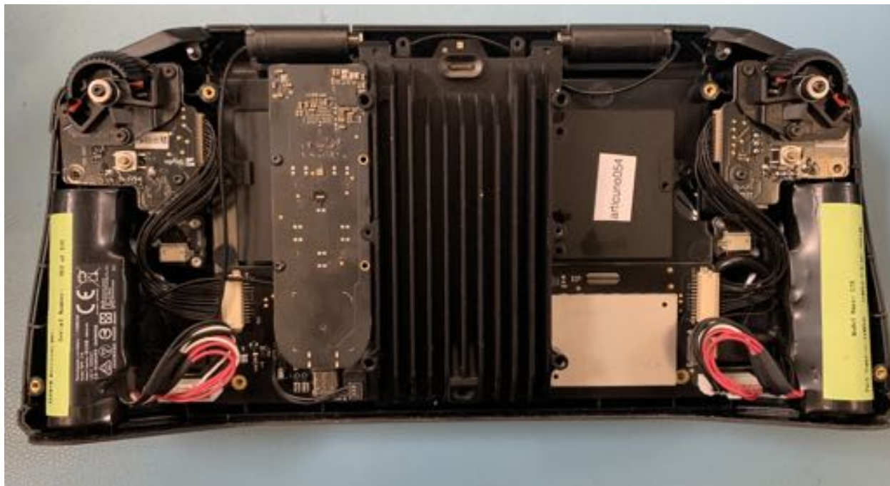
C78 Rear Enclosure Removed, Radio carrier board and MLB visible
