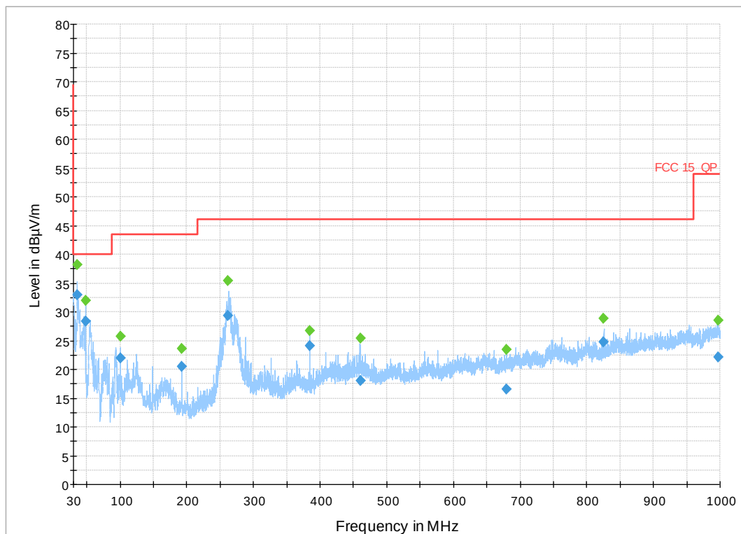
Figure 40: 30 MHz-1 GHz 802.11ac VHT Mode 20 MHz, Mid Channel
