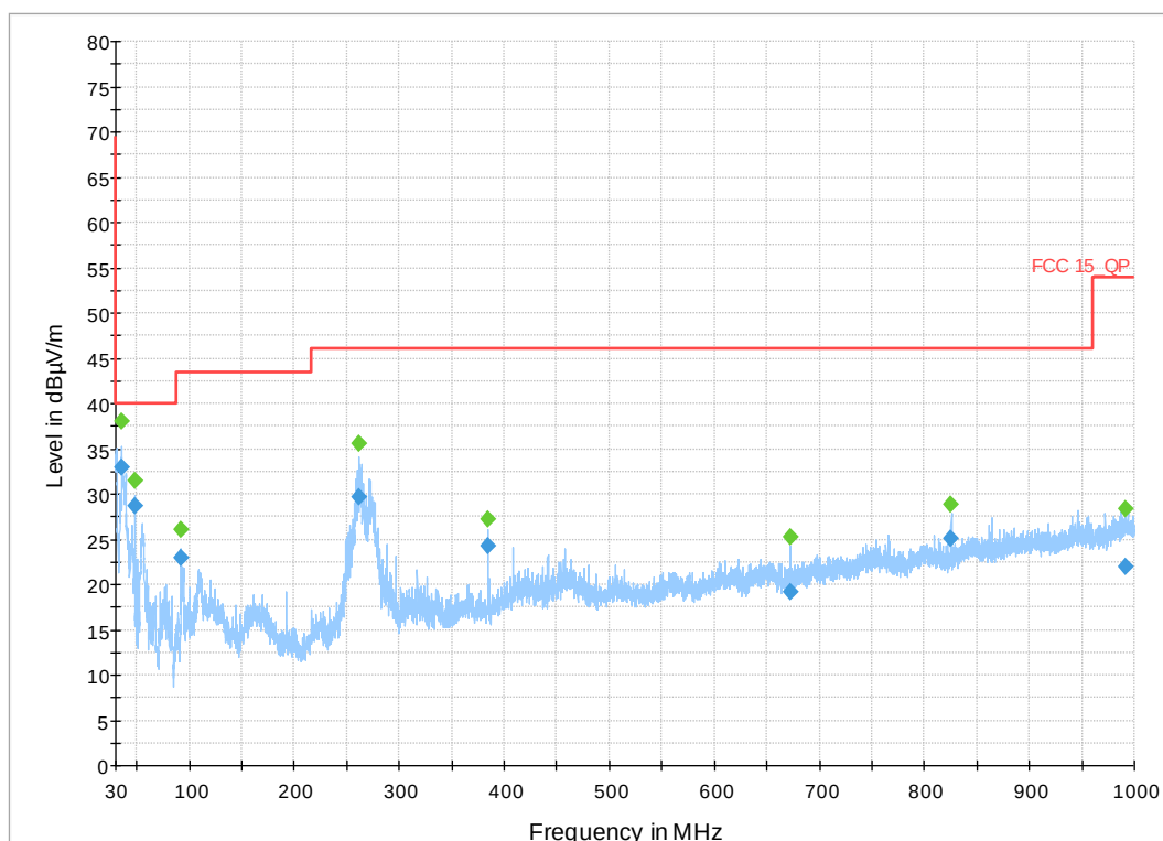
Figure 26: 30 MHz-1 GHz 802.11n HT Mode 10 MHz, Mid Channel
