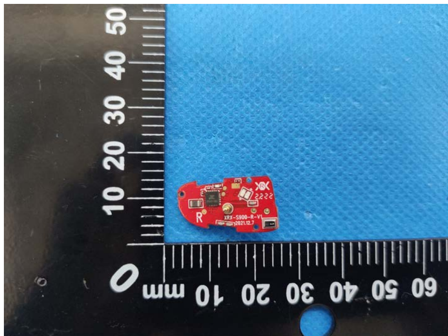
EUT Housing and Board View 8 (Right)
