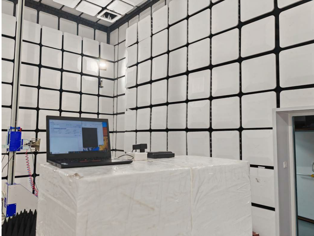
Radiated emission (18-25GHz)
