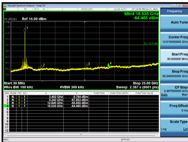
Mode 3 CH00(2402MHz)
