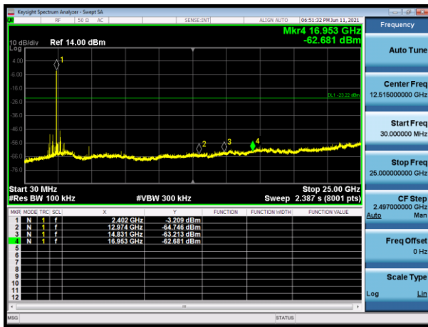
Mode 1 CH00(2402MHz)
