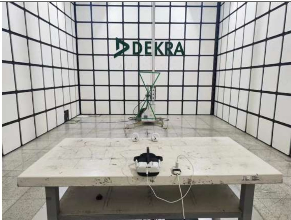
Description: Rear View of Radiated Disturbance Test Setup (Below 1 GHz)
