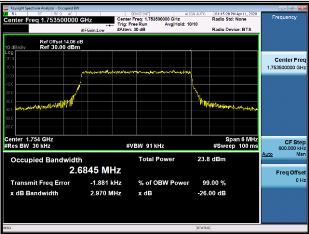
HCH_16QAM_15RB#0
