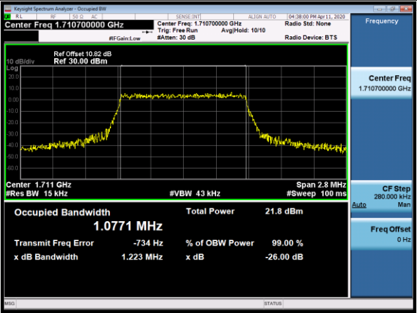
LCH_16QAM_6RB#0
