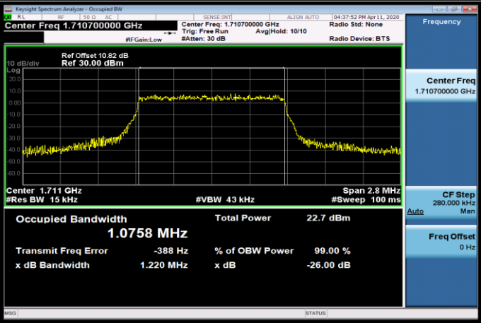
LCH_QPSK_6RB#0
