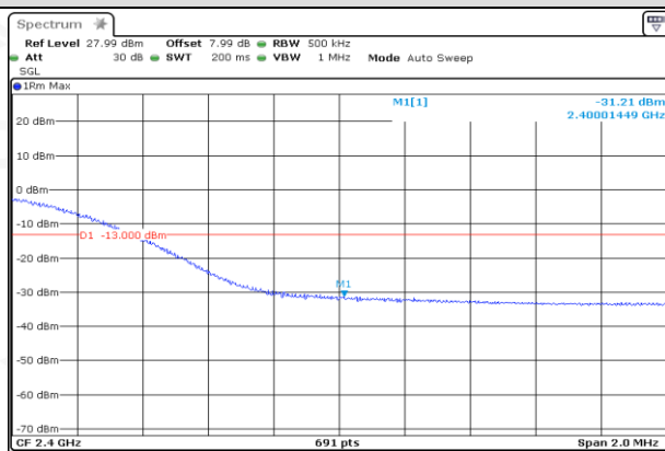
HCH_QPSK_100RB#0
