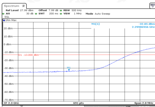
LCH_16QAM_100RB#0
