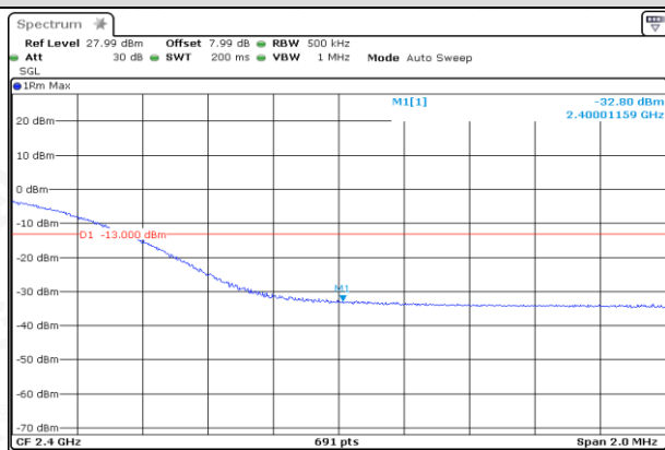
HCH_16QAM_100RB#0
