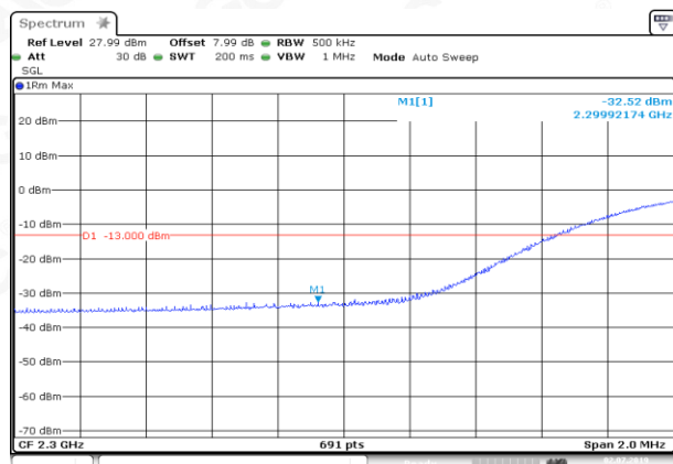
LCH_QPSK_100RB#0
