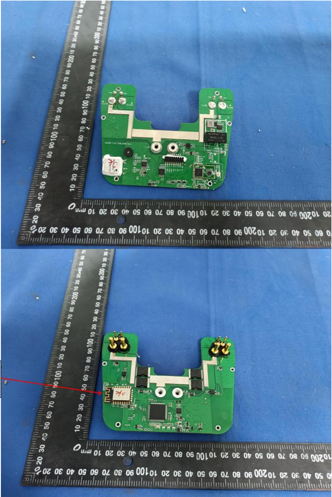
WiFi 2.4G Antenna
