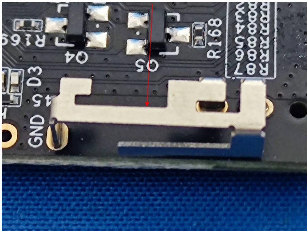
2.4G&5G Wifi Antenna
