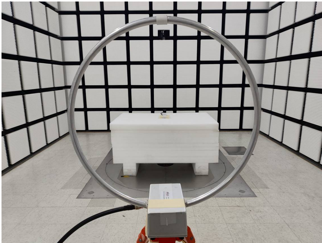
Radiated Emission 9kHz to 30MHz View Parallel
