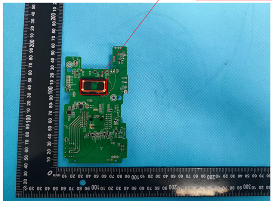
125KHz Antenna
