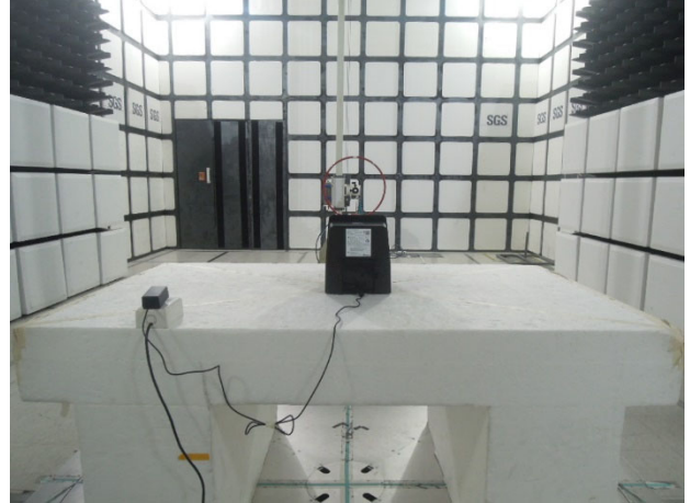
FCC_Part 15.225+RSS 210 NFC_XPS07.1A1_Radiated_Setup
