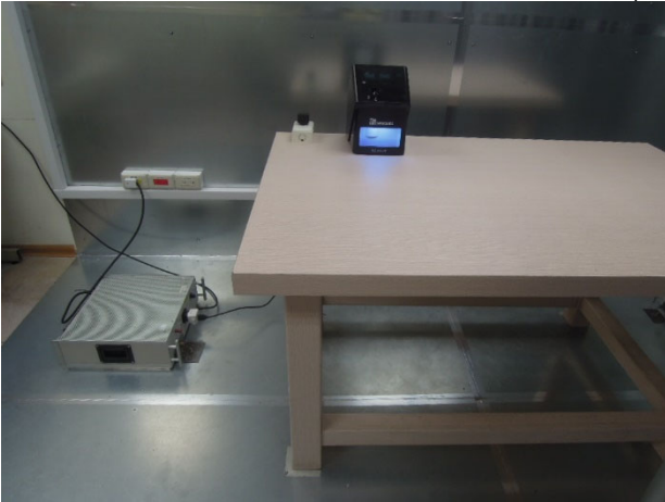
FCC_Part 15.225+RSS 210 NFC_XPS07.2A1_Conduction_setup
