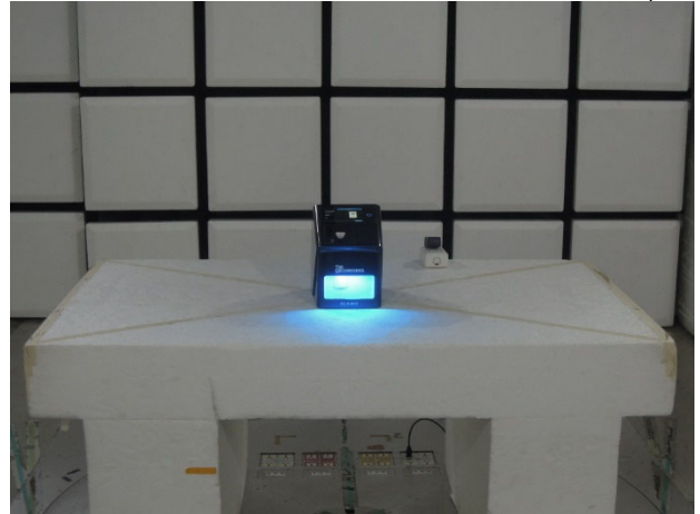
FCC_Part 15.225+RSS 210 NFC_XPS07.2A1_Radiated_Setup
