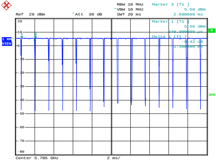
Duty Cycle_11A_5785_Ant2
