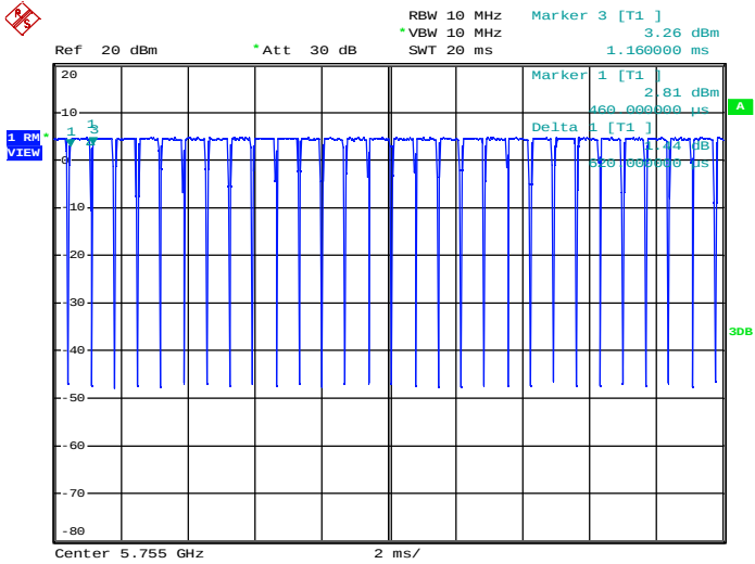
Duty Cycle_11N40_5755_Ant2
