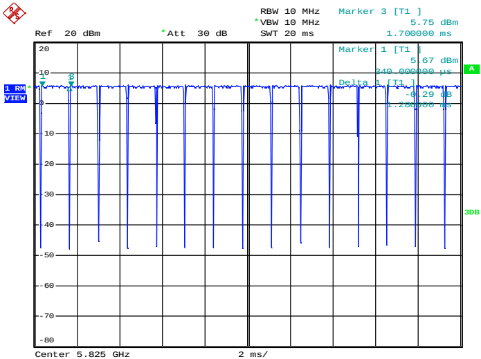
Duty Cycle_11N20_5825_Ant2
