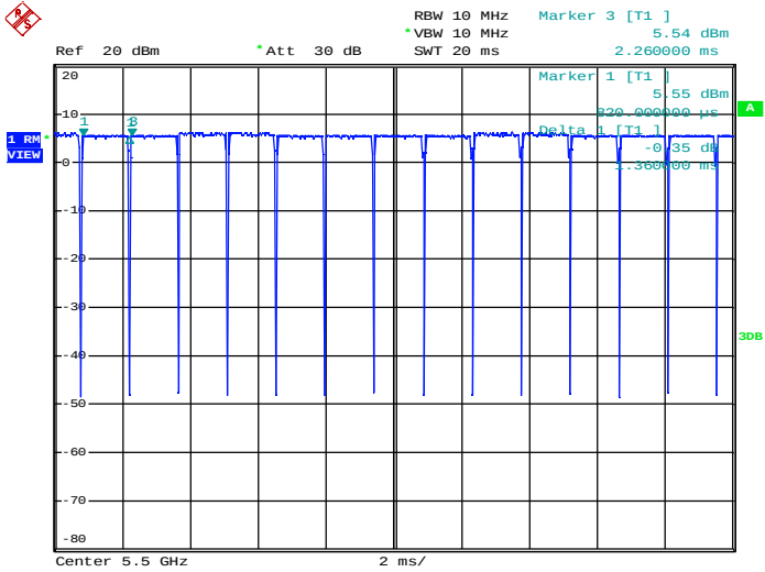
Duty Cycle_11A_5500_Ant2
