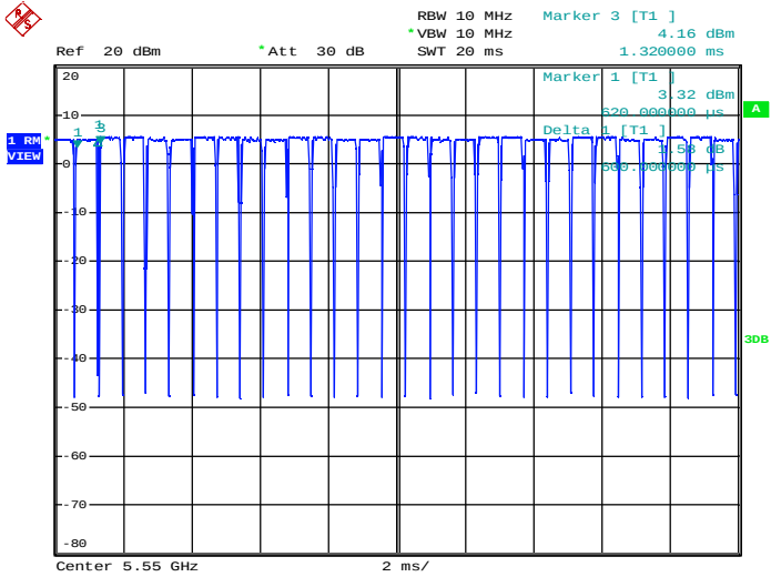
Duty Cycle_11N40_5550_Ant2
