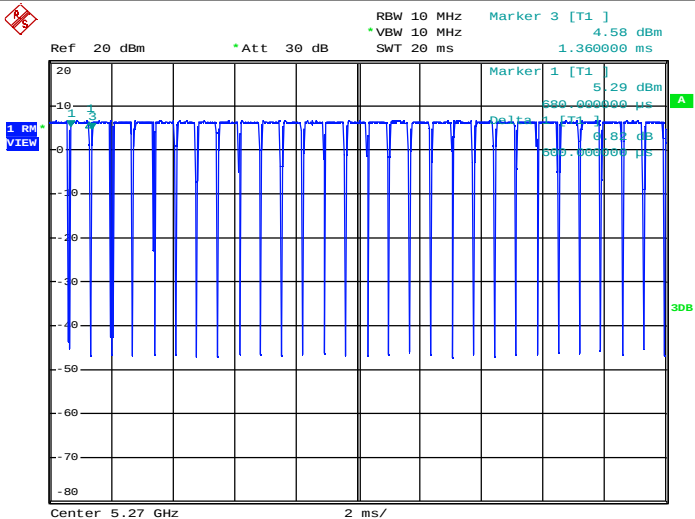
Duty Cycle_11N40_5270_Ant2
