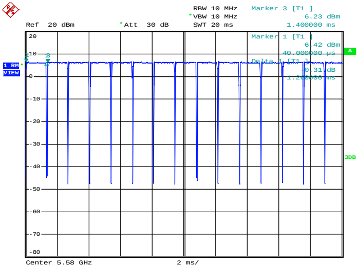
Duty Cycle_11N20_5580_Ant2
