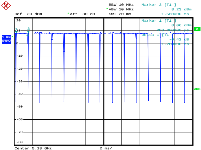
Duty Cycle_11N20_5180_Ant2
