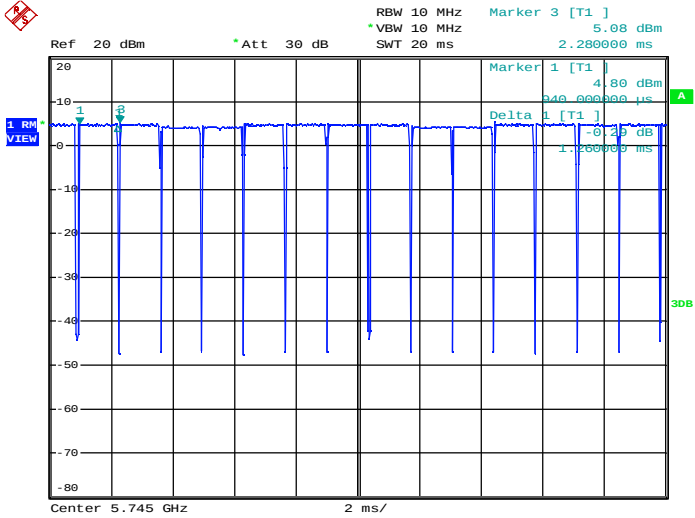
Duty Cycle_11N20_5745_Ant2
