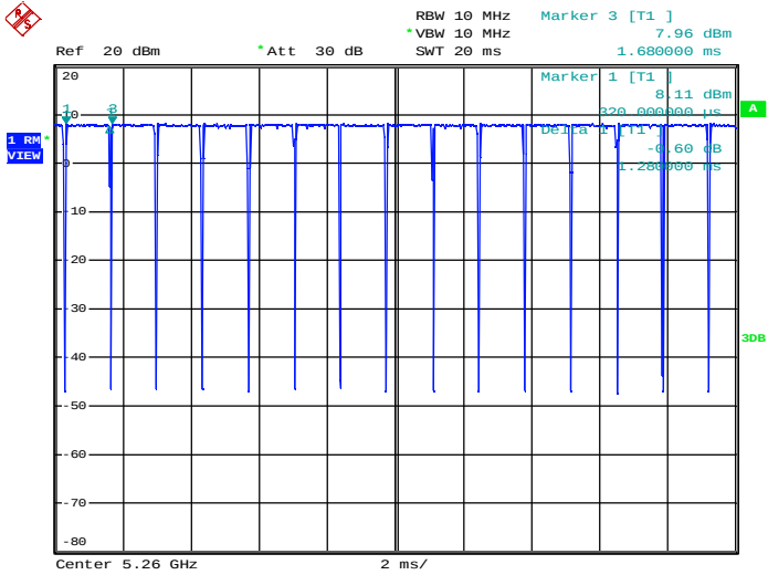
Duty Cycle_11N20_5260_Ant2
