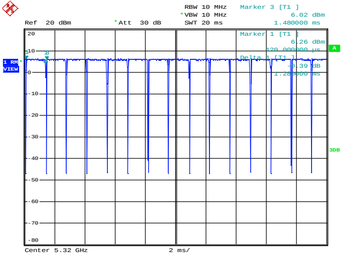
Duty Cycle_11N20_5320_Ant2
