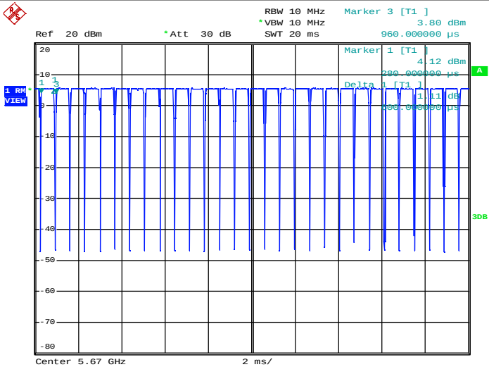
Duty Cycle_11N40_5670_Ant2
