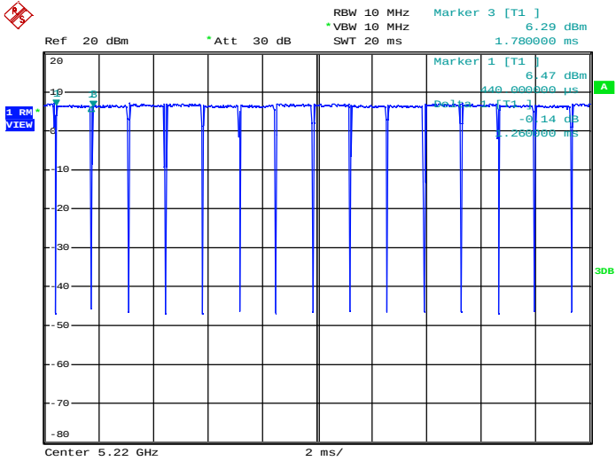
Duty Cycle_11N20_5220_Ant2
