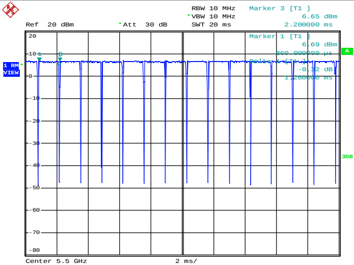
Duty Cycle_11N20_5500_Ant2
