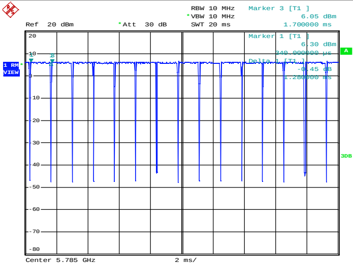
Duty Cycle_11N20_5785_Ant2
