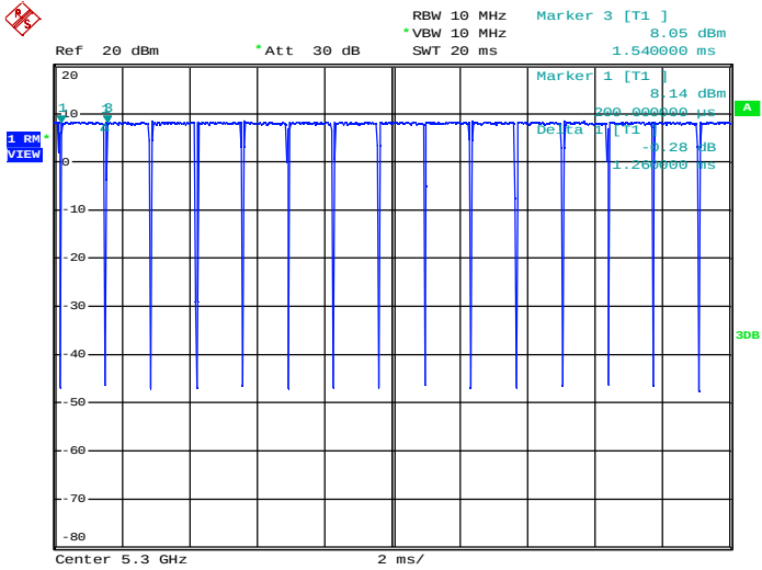
Duty Cycle_11N20_5300_Ant2
