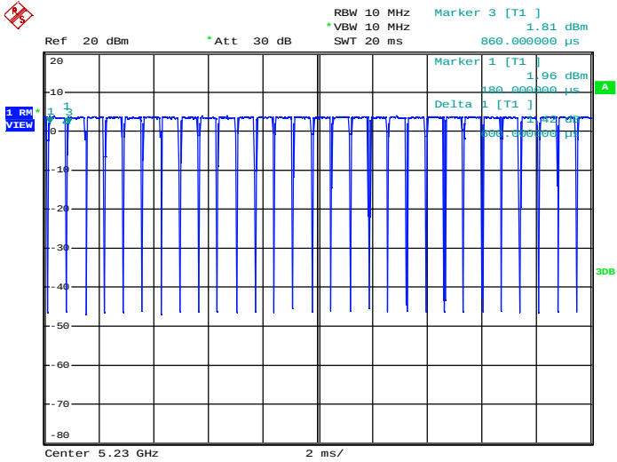
Duty Cycle_11N40_5230_Ant2
