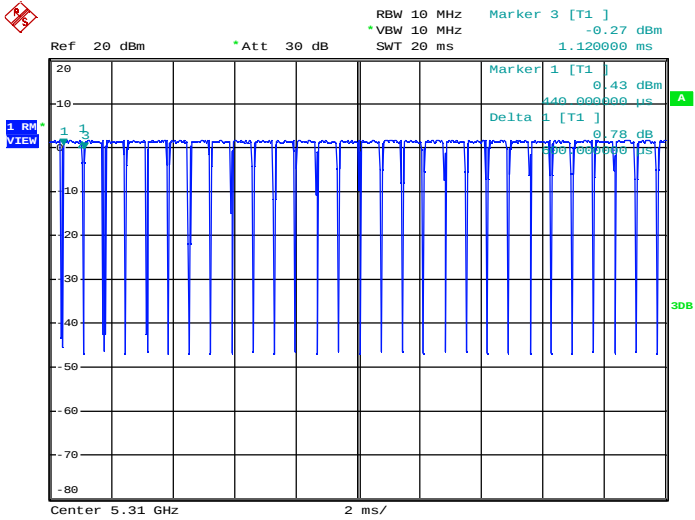
Duty Cycle_11N40_5310_Ant2
