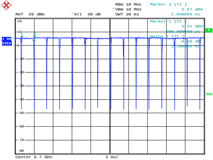
Duty Cycle_11N20_5700_Ant2
