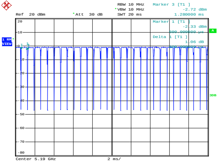
Duty Cycle_11N40_5190_Ant2
