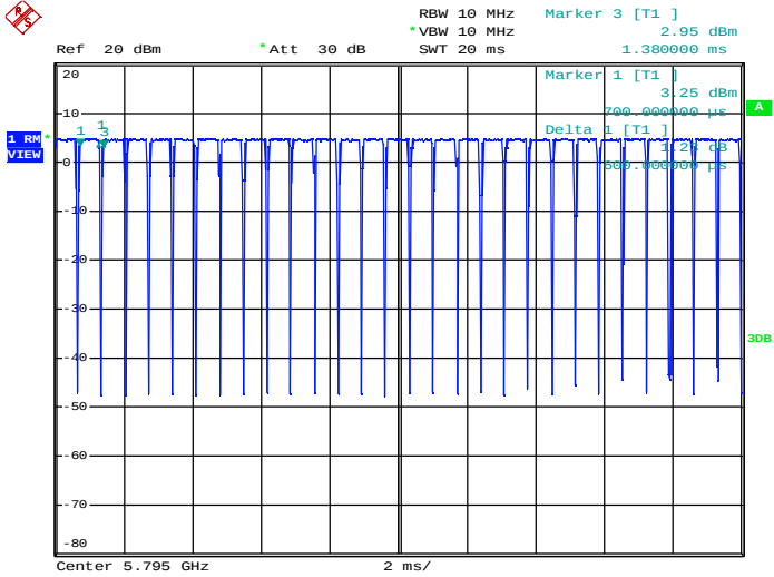
Duty Cycle_11N40_5795_Ant2
