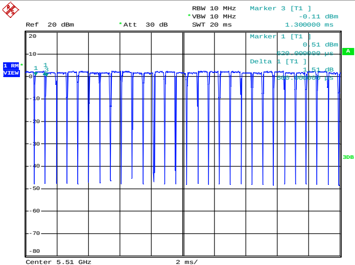
Duty Cycle_11N40_5510_Ant2
